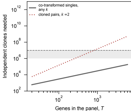
Co-transforming singles instead
