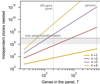
Cloning every combination
