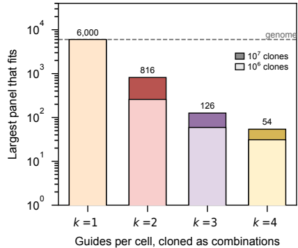
What one transformation buys
