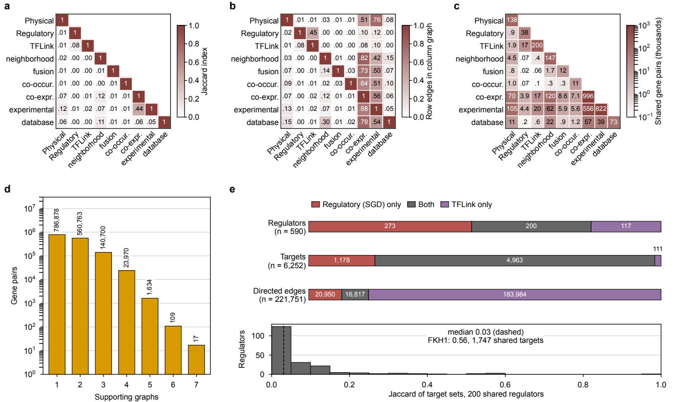
Supplementary Figure 7 How the nine attention-prior graphs relate to each other. Directed graphs are compared as undirected gene pairs; matrix axes in (a)–(c) drop the STRING prefix. (a) Jaccard index of edge sets. (b) Containment: the fraction of the row graph's pairs present in the column graph. (c) Gene pairs shared by each pair of graphs, in thousands (diagonal, the graph's own count; logarithmic color): co-expression and experimental share 556,106 pairs, neighborhood and co-expression 119,758, physical and experimental 104,771, the two transcription-factor graphs 16,885. (d) Distinct gene pairs supported by exactly n graphs (52% in one, 37% in two, none in more than seven); the nine edge sets sum to 2,435,327 pairs, 1,514,071 distinct, 6.9% of the 21.8 million pairs the vocabulary allows. (e) Top: regulators, targets, and directed regulator→target edges of the SGD regulatory graph (473 regulators, 37,767 edges) and TFLink (317 regulators, 200,801 edges), split into one-graph-only (20,950 regulatory, 183,984 TFLink edges) and both (16,817). Bottom: for the 200 shared regulators, the Jaccard index between the regulator's two target sets; the best case is FKH1 at 0.56 (1,747 shared targets). Source: experiments/010-kuzmin-tmi/scripts/graph_statistics.py .
