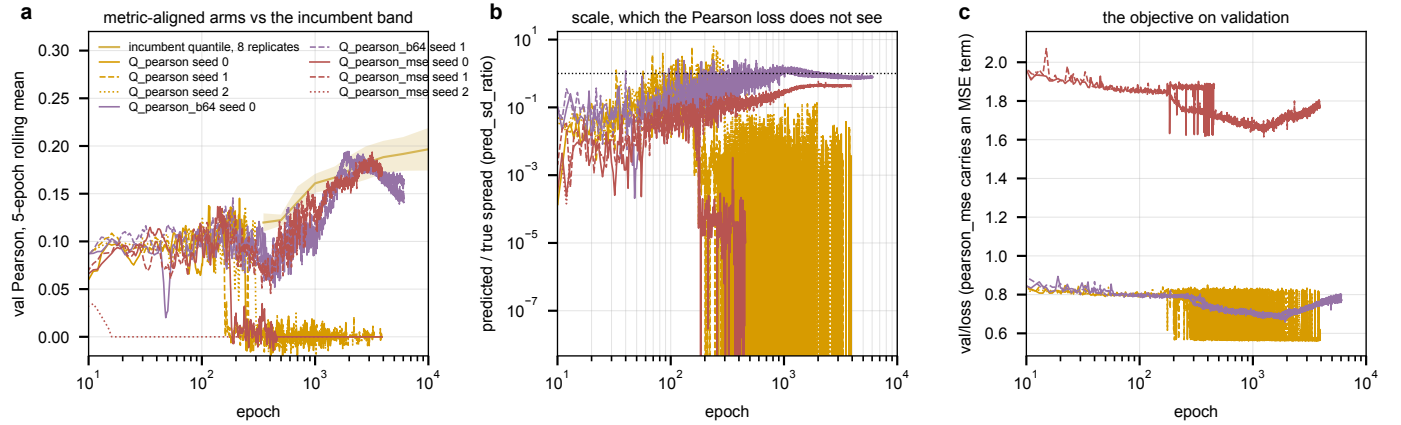
Figure 17: The metric-aligned round at day two. a , validation Pearson of all eight runs against the incumbent replicate band. b , predicted over true spread, which the Pearson loss cannot see; a run whose outputs go constant falls off the bottom. c , the objective on validation; pearson_mse carries the squared-error term and sits on its own scale. Generated by pearson_round_readout.py .
