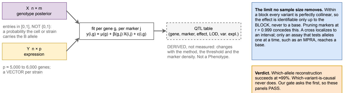
Figure 1: An eQTL study, and where inference enters it. a , The cross. Both parents are deep-sequenced, so the full variant catalog is known before any segregant is examined; the segregants are then assayed twice, sparsely for genotype and densely for expression. b , One chromosome at three levels. True variant sites are dense, observed markers are sparse, and the mosaic between them is an HMM posterior rather than a reading. Crossover positions are localized only to the marker interval, and a non-crossover gene conversion tract falling between markers is missed entirely. c , What is measured against what is derived. The genotype matrix and the expression matrix are measurements; the QTL table is an estimate conditional on the mapping method, the significance threshold and the marker density. Composed from the sources in Sec. 1 rather than redrawn from a published figure; source notes/assets/drawio/eqtl-experiment-and-genotype-inference.drawio .
