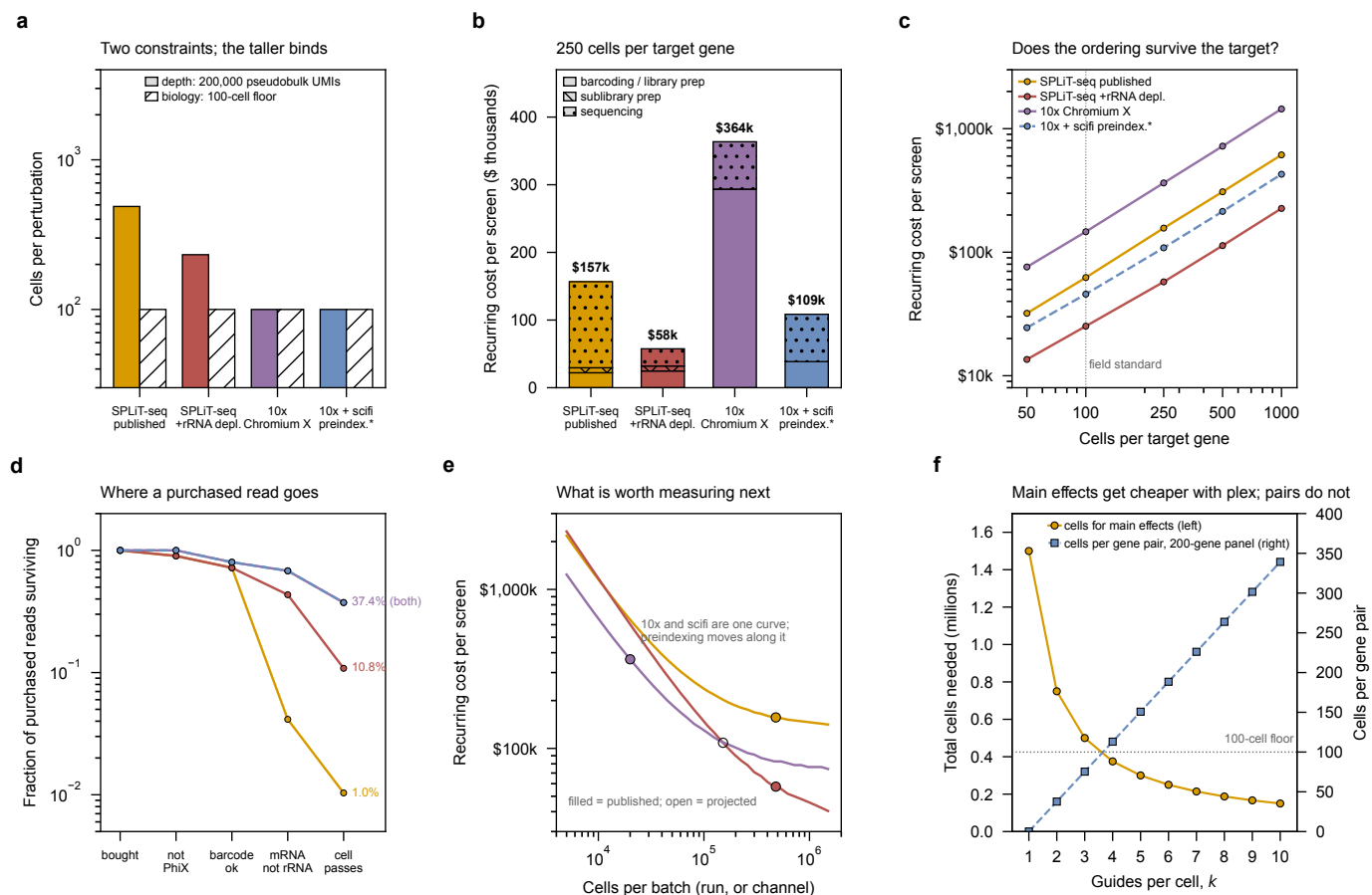
Figure 9: Six views of one decision: which platform to run. Color is the platform in every panel and only ever the platform, so the key is learned once; where a panel needs a second categorical dimension it uses hatching. The asterisk marks the projected row, drawn inside the panels because a screenshot loses a caption. All four columns are 6,000 target genes in one environment at UIUC rates; panels (a), (b), (d) and (e) are priced at 250 cells per target gene. (a) Cells per perturbation, under two independent constraints (section 4.3): the depth requirement, i.e. how many cells it takes to accumulate 200,000 pseudobulk UMIs at each platform's per-cell yield, against the 100-cell biological floor below which cell-cycle and metabolic state are not averaged out. The taller bar binds, and the floor binds for every deeper platform, so past a few hundred UMIs per cell the design is limited by how many cells must be observed rather than by how deeply each is read. The preindexed column is identical to the 10x column here, which is the point of showing it: preindexing buys cells per dollar, not UMIs per cell, and is invisible to every statistical panel in this document (fig. 7d). (b) Where the recurring money goes. The dominant term moves : sequencing is 81% of split-pool spend, while for 10x it is 19% and library preparation 81%, because a genome-scale screen consumes 137 channels at $2,143 each. These are different cost structures, and an optimization that helps one (rRNA depletion, worth ~$99,000 here) does nothing for the other. Preindexing takes the 137 channels to 18 and the column to $109k, and in doing so moves that platform's dominant term onto sequencing as well – reagents 36%, sequencing 64% – but with no rRNA left to deplete. (c) Whether the ordering survives a change of target. Panel (b) prices one design; this sweeps 50 to 1,000 cells per target gene. The ordering is stable across the whole range, so the platform choice is not an artifact of the 250-cell point, and the vertical rule marks the 100-cell field standard the recommendation is actually made at. (d) What happens to a purchased read , stage by stage, and this is where the reagent comparison and the cost comparison part company. Split-pool reagents are ~22× cheaper per cell than droplet and it still loses end to end; the reversal is entirely here. Of 100 reads bought for a split-pool run, 10 are PhiX spike or unresolvable barcode, 94 of the remainder are ribosomal, and three quarters of the cells they came from are then discarded – 1.0 read in 100 survives all four tolls. Depletion takes that to 10.8, and both droplet columns reach 37.4. The two droplet lines coincide exactly at every stage , which is worth seeing: preindexing touches no term in this panel. (e) What is worth measuring next. Every platform here has exactly one number that is both uncertain and load-bearing, and for all of them it is the same field – cells barcoded per protocol run, or cells recovered per channel – so they share an axis. The two are not equally worth measuring. Droplet cost is reagents and reagents are per batch, so its curve falls steeply and keeps falling; split-pool cost is sequencing, which does not depend on this number at all, so its curve flattens almost at once and learning that yeast tolerates a denser RT well buys little past a few hundred thousand cells per run. 10x and scifi are one curve, and preindexing is a move along it rather than a move to a different one. (f) What multiplexing buys as guides per cell k rises. Left axis: total cells needed to hold main-effect precision across 6,000 genes falls as 1/k , from 1.5M cells at k = 1 to 0.15M at k = 10 , because every cell reports on k genes at once. Right axis: what that same cell budget delivers for one named gene pair if the library is restricted to a 200-gene panel, which grows roughly linearly in k and crosses the 100-cell floor near k = 4 . Multiplexing alone does not open up epistasis – run the same calculation over all 6,000 genes and coverage per pair falls by (200/6000)^2 \approx 1/900 , to well under one cell per pair at any k , because the pairs to be covered grow quadratically while the pairs a cell reports grow only as k^2 . Restricting the panel is what makes pairs measurable and multiplexing is what then makes it affordable; neither substitutes for the other. The scifi column is a projection throughout. It changes exactly one parameter of the 10x column – cells recovered per channel becomes Datlinger et al.'s measured 151,788 rather than the UIUC baseline of 20,000 – and per-cell depth in yeast is unmeasured for that chemistry and held at the 10x value, the optimistic end. No scifi run in any microbe has been published (section 3.3). Every panel is generated by experiments/019-per22-urb-seq-costing/scripts/plot_economics.py , which fails rather than writing the figure if any two labels in it collide.
