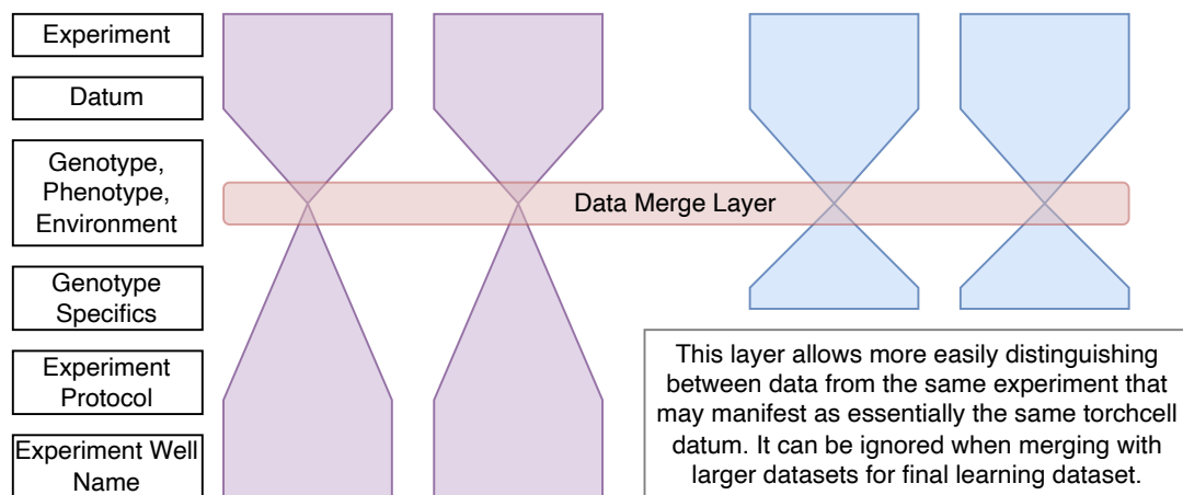
Supplementary Figure 14 Ontology data model (hourglass). Each experiment funnels genotype, phenotype, environment, and experiment-specific metadata through a shared Data Merge Layer that distinguishes records from the same experiment; the layer can be ignored when merging into larger datasets.
