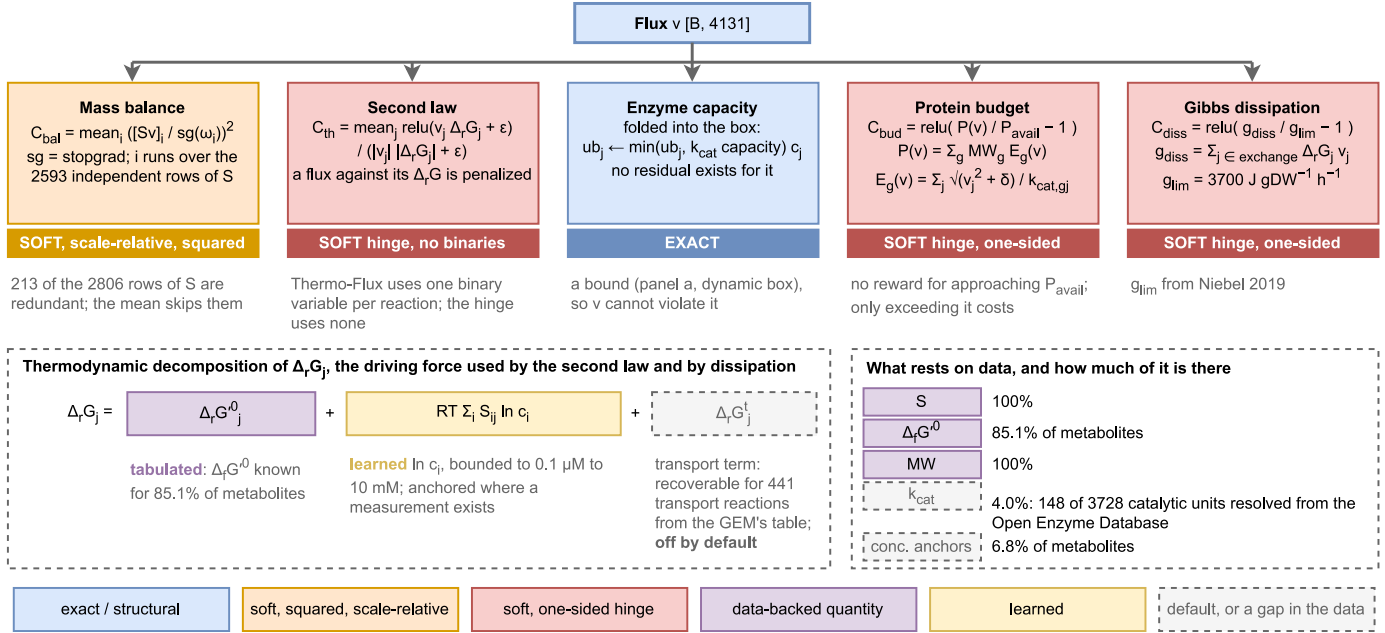
Figure 3. The flux layer, from gene tokens to a feasible flux vector and its residuals. (a) A deletion sets gene availability to zero as a hard fact, not a learned gate; complexes take a softmax over subunits and isozymes sum, and enzyme capacity enters the bounds rather than the loss, so the box holds by construction and contributes no loss term. (b) Five residuals hang off the flux. One is exact and the other four are smooth penalties, none requiring a binary variable. The insets give the three-term decomposition of the reaction driving force and the fraction of each input that is measured rather than defaulted.
