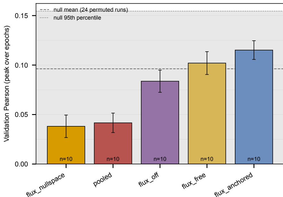
Figure 6. Every arm sits inside the noise band. Bars are the mean maximum validation Pearson for betaxanthin across ten seeds, error bars the standard error. The dashed line is the mean of 24 label-permutation runs and the dotted line their 95th percentile; the shaded region is everything below that percentile. No arm clears it, and the smallest p-value across all 22 configurations tested is 0.24.
