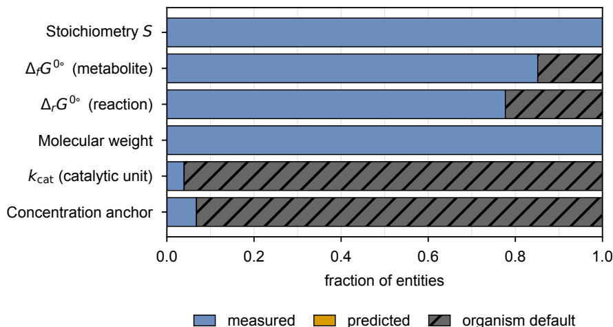
Figure 2. What each parameter class rests on: measurement, prediction, or an organism default. Stoichiometry and molecular weight are complete and formation energies cover most metabolites, but turnover is resolved for only 4.0 percent of catalytic units from the Open Enzyme Database and nothing is predicted yet. A capacity constraint built on a default turnover is a uniform rescaling of the flux box rather than an enzyme constraint, and no loss curve distinguishes the two.
