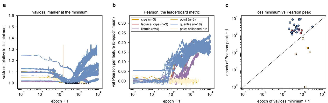
Figure 2: The validation loss bottoms out before the Pearson peaks in every run, so the long budget buys Pearson on a rising objective. a , validation loss relative to its minimum, one curve per run, colored by head; pale curves are collapsed runs. b , the 5-epoch rolling mean of validation Pearson. c , the epoch of the loss minimum against the epoch of the Pearson peak; every point lies above the diagonal. Generated by loss_min_vs_pearson_peak.py .
