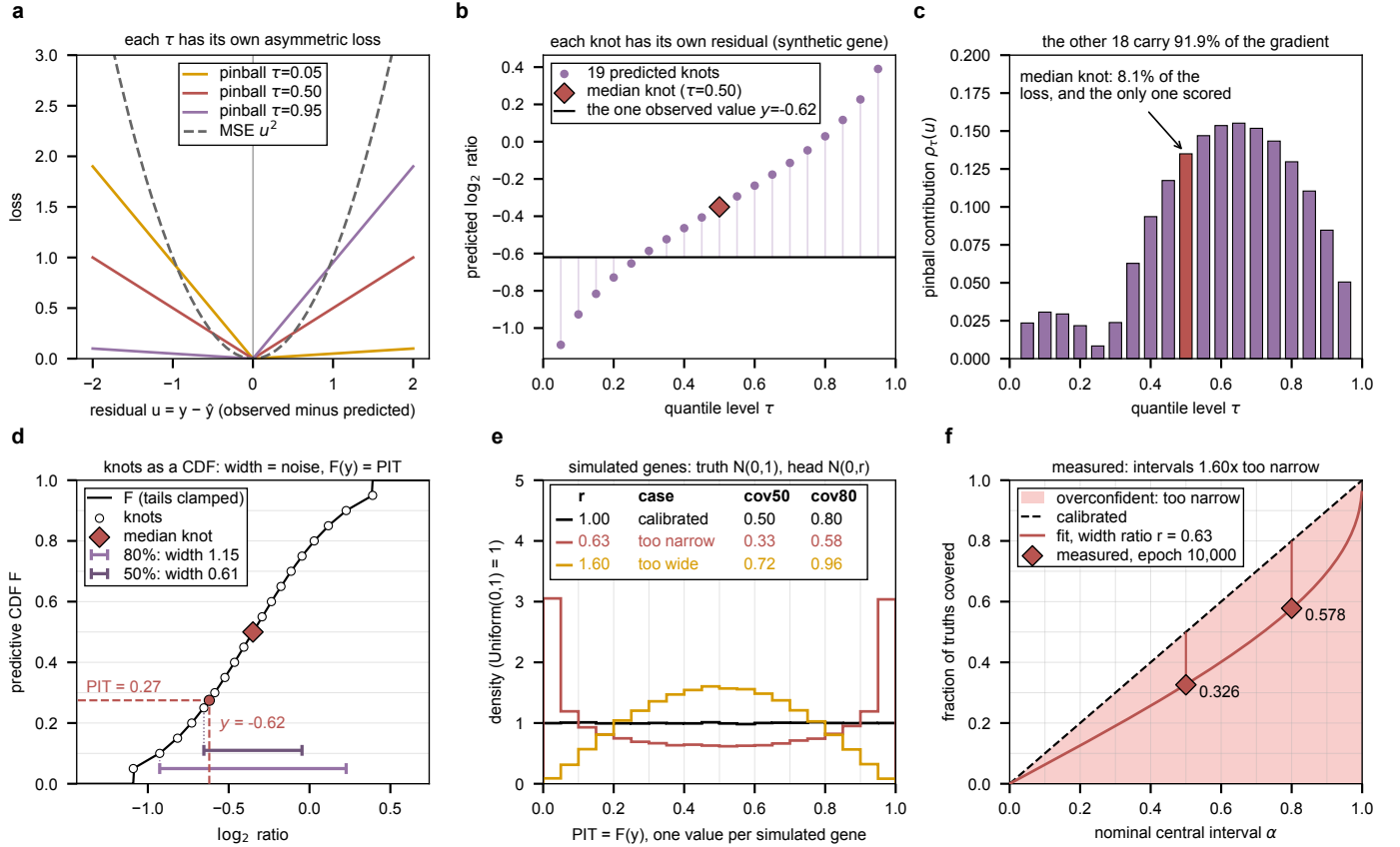
Figure 1: The metric reads one knot of nineteen, and the eighteen it ignores set intervals the incumbent makes 1.6 times too narrow. Panels a to e are synthetic; f is measured. a , the pinball loss at three quantile levels against squared error. b , one illustrative gene: 19 predicted knots, the median knot, and the one observed value; each knot's residual to that value feeds its own pinball term. c , the 19 terms; the median carries 8.1% and is the only knot the metric scores. d , the same knots read back as a CDF (joined piecewise-linearly, tails clamped as _quantile_pit does): the central 80% and 50% interval widths are the model's own noise estimate for that gene, and the CDF at the observed value is its PIT. e , PIT histograms over 200,000 simulated genes with truth N(0,1) and a head predicting N(0,r) : flat when r = 1 , U-shaped when the intervals are too narrow, humped when too wide, with the coverage of the central 50% and 80% intervals per case. f , the incumbent's measured coverage at epoch 10,000 as a reliability curve; the fitted curve is a single width ratio r = 0.63 , derived not measured. Generated by plot_pinball_vs_mse.py .
