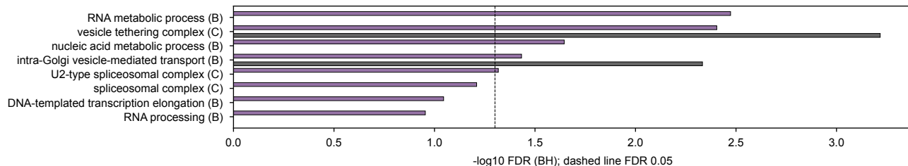
acetic acid: Hoepfner HOP sodium acetate vs acid prediction
