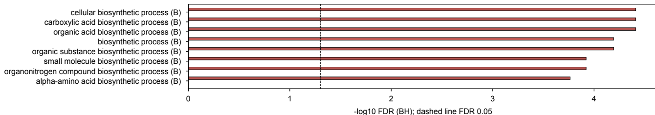
acetic acid: Hoepfner HOP sodium acetate vs acid prediction
