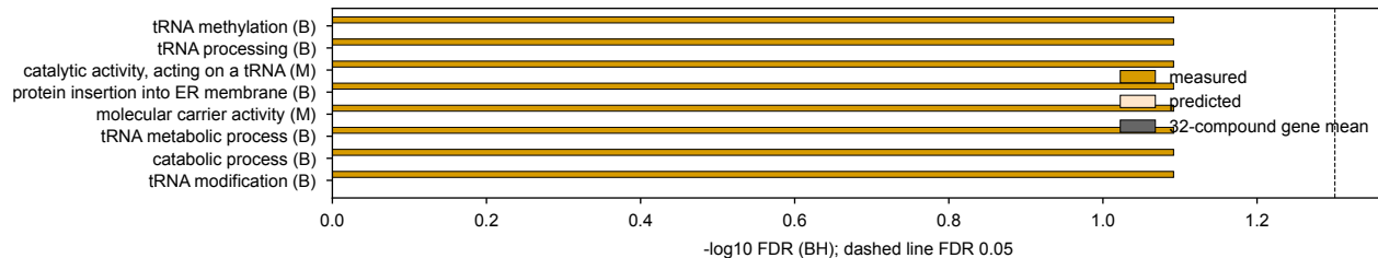
5-HMF: measured b002 (reliability -0.05) vs LOCO prediction
