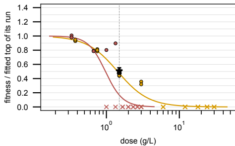
formic acid (FA)
