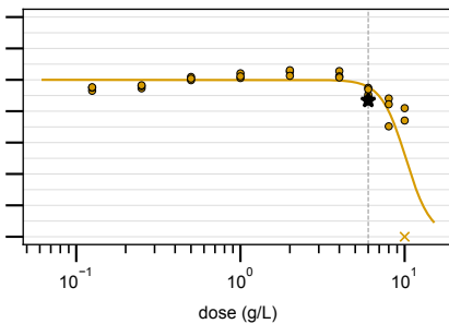
levulinic acid (LVA)
