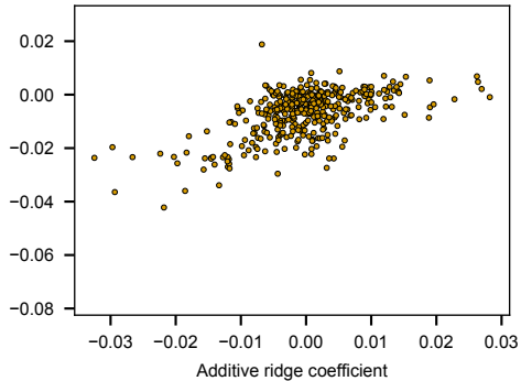
inference 1, r = 0.579
