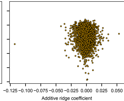
inference 3, r = -0.008
