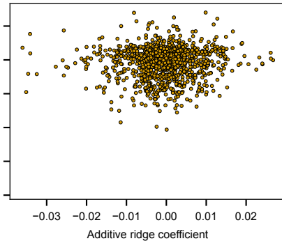
inference 2, r = 0.048
