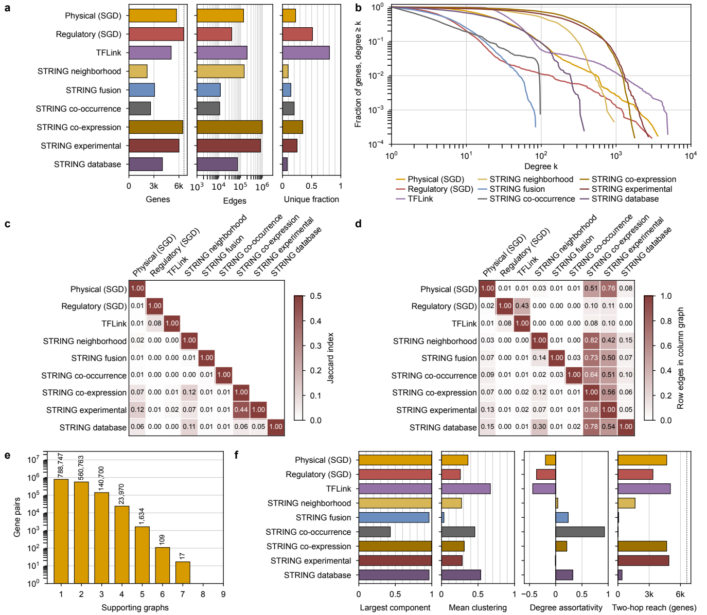
Supplementary Figure 6 Gene-gene graphs used as attention priors in the trigenic experiment. Directed graphs (regulatory, TFLink) are compared as undirected gene pairs. (a) Genes with at least one edge (dotted line, the 6,607-gene reference), distinct gene pairs, and the fraction of each graph's pairs found in no other graph. (b) Complementary cumulative degree distribution over undirected gene pairs: fusion and co-occurrence have no gene above degree 100, the two dense STRING channels fall off past degree 10 3 , and TFLink carries the heaviest tail. (c) Jaccard index of edge sets. (d) Containment: the fraction of the row graph's pairs present in the column graph. (e) Distinct gene pairs supported by exactly n of the nine graphs (52% in one graph, 37% in two); the nine edge sets sum to 2,437,196 pairs, of which 1,515,940 are distinct, 6.9% of the 21.8 million pairs the vocabulary allows. (f) Per graph: fraction of covered genes in the largest connected component (96% to 100% for all but co-occurrence, 43%), mean clustering coefficient (0.03, fusion, to 0.67, TFLink), degree assortativity (negative for the three curated graphs, TFLink -0.44, regulatory -0.37, physical -0.20; 0.93 for co-occurrence; -0.01 for experimental), and the mean number of genes within two edges of a gene (dotted line, the 6,607-gene reference); the four dense graphs place over 70% of the vocabulary within two edges of a typical gene, fusion and co-occurrence under 2%. Source: experiments/010-kuzmin-tmi/scripts/graph_statistics.py .
