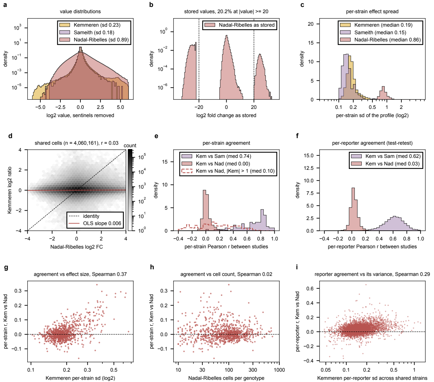
Figure 7: Three single-deletion expression panels compared, base medium only. a , \log_2 values of each panel with the Nadal-Ribelles sentinels removed; the two platforms sit on different scales. b , Nadal-Ribelles values as stored, with the \pm 20 lines: 20.2% of cells are the zero-mean sentinel. c , per deletion, the standard deviation of its profile across reporters. d , Kemmeren against Nadal-Ribelles on every shared (strain, gene) cell, log-count density, with the identity and the fitted slope. e , per shared deletion, the Pearson across reporters between its two profiles: Kemmeren vs Sameith ( n = 82 ), Kemmeren vs Nadal-Ribelles ( n = 914 ), and the latter over only the reporters with |\log_2| > 1 in Kemmeren (dashed, n = 368 strains). f , per reporter, the Pearson across shared strains between its two response vectors, the test-retest reliability behind the ceiling. g , the per-strain agreement of e against the strain's Kemmeren spread; h , against the number of cells behind its pseudobulk; i , the per-reporter agreement of f against the reporter's Kemmeren spread across the shared strains. Generated by cross_study_ko_expression.py .
