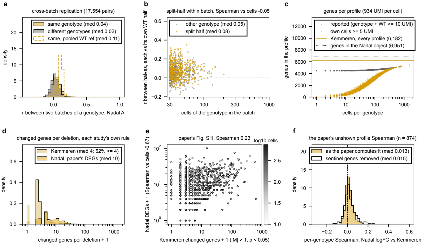
Figure 10: Within-study replication, coverage, and the paper's own deleteome comparison. a , Pearson between two batches of one genotype (pseudobulk against the batch's own wild-type cells), the different-genotype null with matched cell counts, and the same-genotype value with a pooled wild-type reference. b , split-half within one batch, each half against its own half of the wild-type cells, against cells per genotype; gray, the other-genotype null. c , genes per profile: covered by the genotype's own cells at five or more UMI, and reported under the summed-UMI rule; lines at Kemmeren's reporters per profile and at the genes in the single-cell object. d , changed genes per deletion under each study's own rule. e , the paper's Supplementary Fig. 1i reproduced from its released objects, shaded by cells per genotype. f , the per-genotype profile Spearman the paper's script computes and does not show, with and without the sentinel genes. Generated by nadal_replication_coverage.py from nadal_batch_replication.R and nadal_paper_deleteome_comparison.R .
