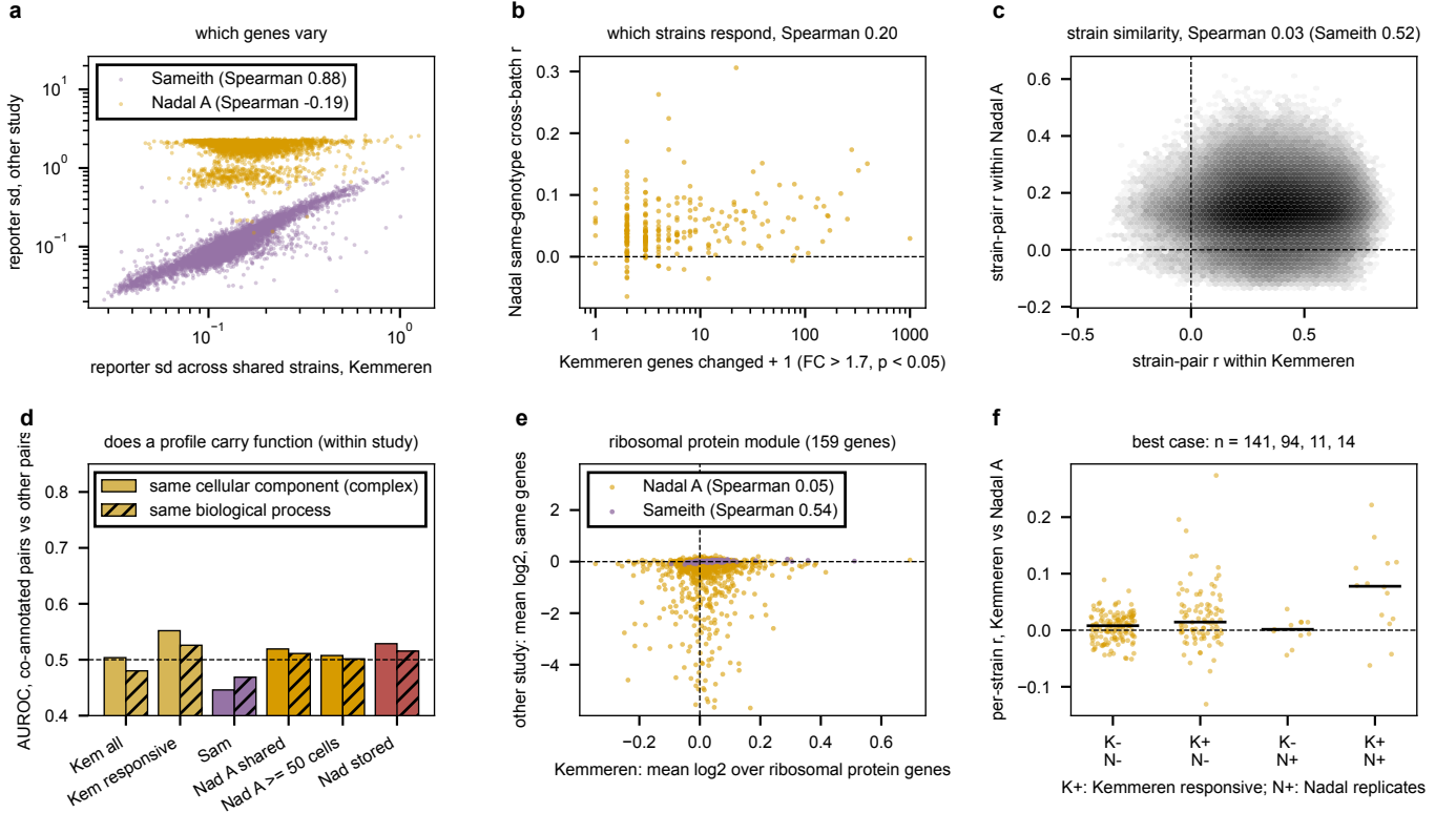
Figure 11: Agreement at levels a per-gene correlation misses, on the 1,002 shared deletions. a , a reporter's sd across the shared strains, Kemmeren against Sameith and against Nadal-Ribelles A. b , Kemmeren's changed-gene count per deletion against the genotype's cross-batch replication in Nadal-Ribelles A. c , strain-pair correlation within Kemmeren against the same pair within Nadal-Ribelles A. d , within one study, the AUROC of the pair correlation for pairs annotated to one GO cellular-component or biological-process term of 5 to 100 genes against other pairs. e , mean log 2 over 159 cytosolic ribosomal protein genes per strain, Kemmeren against Nadal-Ribelles A and against Sameith. f , per-strain cross-study r by whether Kemmeren calls the deletion responsive (K+) and whether its Nadal-Ribelles profile replicates across batches at r \geq 0.1 (N+); bars are medians. Generated by cross_study_structure.py .
