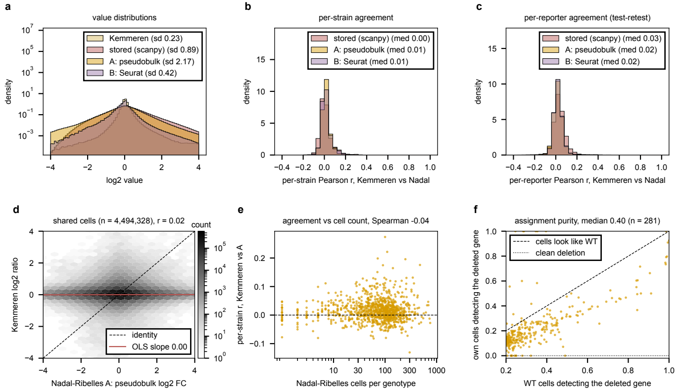
Figure 8: Recomputing the Nadal-Ribelles fold change from the single-cell object, and why it does not help. a , \log_2 values of Kemmeren and of three Nadal-Ribelles versions: as stored, the bulk-like pseudobulk ratio (A) and Seurat's avg_log2FC (B). b , per shared deletion, the Pearson across reporters with Kemmeren for each version; c , the same per reporter across shared strains. d , Kemmeren against A on every shared cell. e , per-strain agreement of A against the cells behind the genotype. f , assignment purity: for each genotype whose deleted gene wild type detects in at least a fifth of cells, the fraction of the genotype's own cells detecting that gene against the wild-type fraction; the dashed identity is what cells that are not the genotype look like, the dotted zero a clean deletion. Generated by cross_study_recomputed.py from nadal_pseudobulk_recompute.R and nadal_assignment_purity.R .
