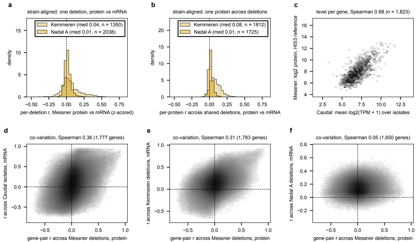
Figure 12: The Messner 2023 knockout proteome against three expression panels. a , per shared deletion, the Pearson between its protein and mRNA \log_2 ratios (z-scored per gene across strains) for Kemmeren and for Nadal-Ribelles A. b , per protein, the Pearson across shared deletions. c , abundance level per gene, protein in the HIS3 reference against mean expression over the Caudal isolates. d–f , gene-pair co-variation: the correlation of two genes across Messner’s deletions (protein) against the same pair across Caudal’s isolates, Kemmeren’s deletions and Nadal-Ribelles A’s deletions (mRNA), log-count density. Generated by proteome_expression_covariation.py .
