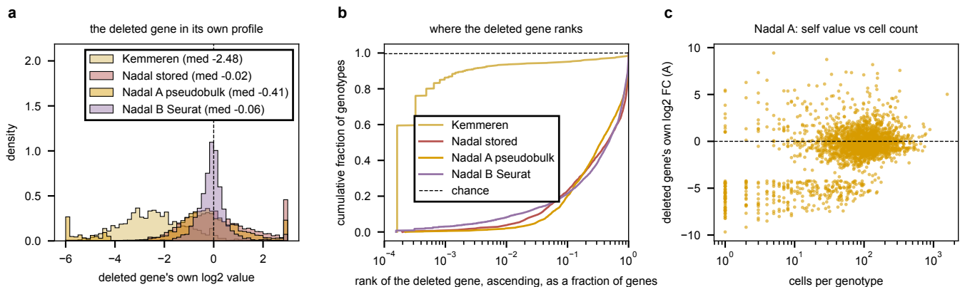
Figure 9: The deleted gene in its own profile. a , the deleted gene's own \log_2 value per genotype for Kemmeren and three Nadal-Ribelles statistics. b , cumulative distribution of the deleted gene's ascending rank as a fraction of genes in the profile, log axis; the dashed diagonal is chance. c , for the pseudobulk statistic, the deleted gene's own value against the cells behind the genotype; the band near -5 to -8 at low counts is the pseudocount floor of a near-empty pseudobulk. Generated by nadal_identify_deletion.py .
