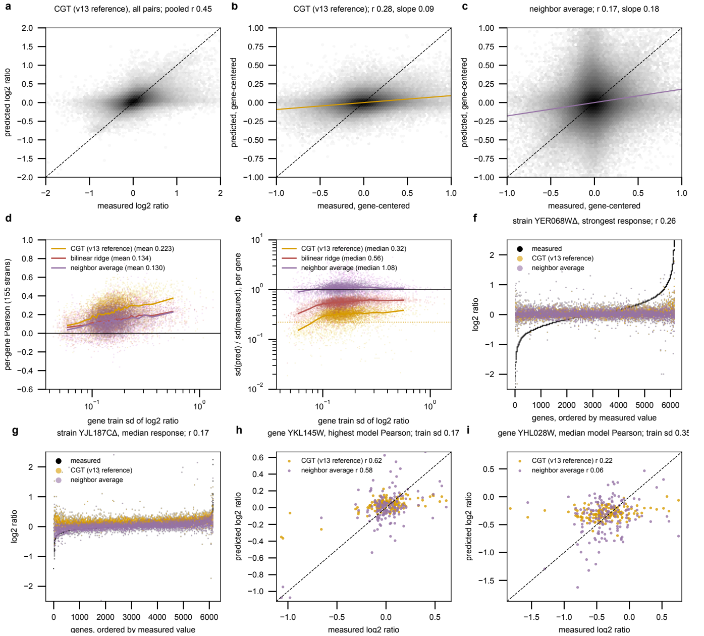
Figure 5: The v13 reference predicts the direction a gene moves across strains and not the distance; the large responses are missing from every predictor. Validation strains of split seed 0 on fig3_core (155 strains, 6,127 graph genes). CGT: v13 reference checkpoint, run wq8y8nd5; ridge and neighbor average: B2 and B3 on ProtT5, cells selected on validation. a , Predicted against measured log2 ratio, every strain-gene pair (hexbin, log count); pooled Pearson 0.45. b , The same with each gene's train mean removed from both axes; pooled Pearson 0.28, regression slope 0.09 (orange). c , The neighbor average on the axes of b ; 0.17, slope 0.18. d , Per-gene Pearson over the 155 strains against the gene's train sd, with the running median per predictor (40 bins); means 0.223, 0.134, 0.130. e , Per-gene sd(pred) / sd(measured) on the same axis; the solid line is 1, the dotted line 0.22 is the model's mean Pearson; medians 0.32, 0.56, 1.08. f , g , One strain each, genes ordered by the measured value: the strongest-response strain (YER068W deletion, sd over genes 0.56, per-strain Pearson 0.26) and a median one (YJL187C deletion, 0.17, 0.17). h , i , One gene each over the 155 strains: the gene with the highest model Pearson (YKL145W, 0.62; neighbor average 0.58) and the gene at the model's median (YHL028W, 0.22; 0.06). Dashed lines are the identity. One checkpoint, one partition; no uncertainty is shown.
