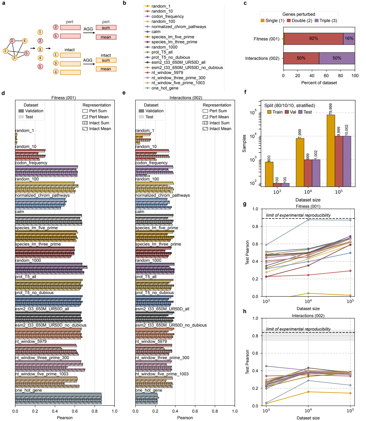
Supplementary Figure 4 Classical machine-learning baselines: fitness is saturable, interactions are not. a , Featureization. Each strain is reduced to a single fixed-length vector by mapping its genes through a per-gene encoder and pooling: the bag is taken over either the perturbed (deleted) genes or the intact genome and aggregated by sum or mean. b , The seventeen gene representations, grouped as identity (one-hot), random projections ( d=1 – 1000 ), hand-crafted (codon frequency, chromosome/pathway features), and pretrained biological encoders (CaLM, a species-aware DNA language model [16], nucleotide-transformer windows, ProtT5, ESM2). c , Perturbation composition of the two datasets: knockout fitness (001; single/double/triple deletions) and the digenic/trigenic interaction mixture (002). (d,e) Validation and test Pearson r at n=10^5 for random forest across all representations and the four pooling variants (perturbed/intact \times sum/mean), hyperparameters selected on validation MSE; Spearman and MSE views, and the support-vector and elastic-net baselines, are tabulated in Supplementary Table 3–5. f , Stratified 80/10/10 train/validation/test splits at each dataset size. (g,h) Best test Pearson r per representation as dataset size grows n=10^3 – 10^5 ; the dashed line and shaded band mark the limit of experimental reproducibility (fitness r \approx 0.89 ; interactions r \approx 0.81 – 0.86 ). Fitness is saturated by gene identity – one-hot reaches Pearson \approx 0.87 at n=10^5 , approaching the reproducibility limit, and no pretrained embedding surpasses it – whereas interactions plateau near Pearson \approx 0.4 regardless of representation or scale, the empirical backing for the information-accounting cut of Supplementary Note 5.
