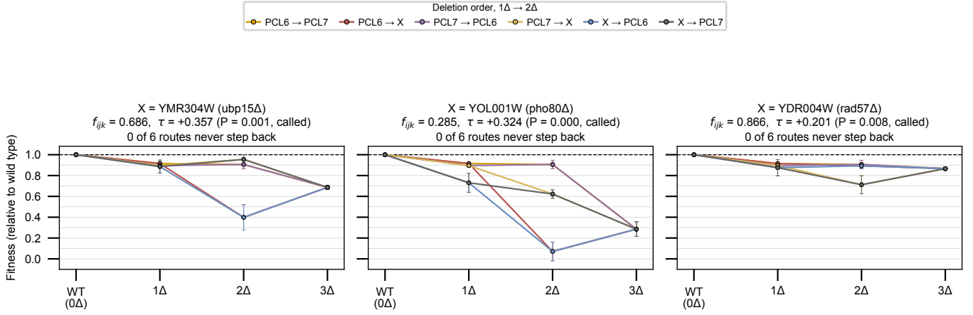
Figure 4: Every triple in the screen clearing the strong positive tier, all six deletion orders each. Generated by experiments/010-kuzmin-tmi/scripts/pcl6_deletion_paths.py .
