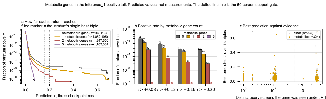
Figure 7: How far each metabolic stratum reaches into the positive tail, the positive rate at each cut with counts labeled including the zeros, and each gene's best prediction against the number of distinct query screens it was seen under. Generated by experiments/010-kuzmin-tmi/scripts/metabolic\_positive\_predictions.py .
