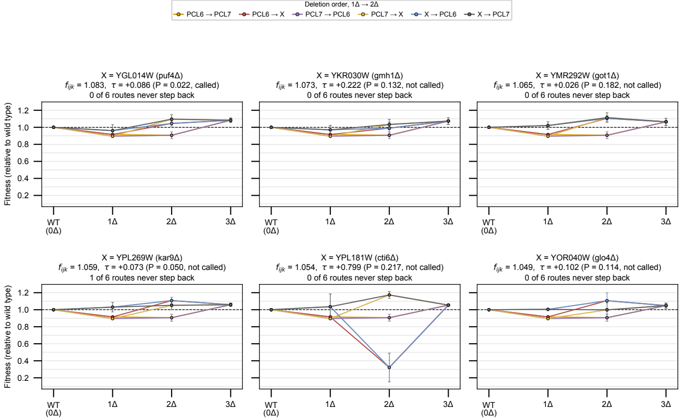
Figure 6: The six highest-fitness triples of the screen, all six deletion orders each, error bars 1 SE. Two of the six routes pass through the paralog double, whose fitness is one value for the whole screen. Generated by experiments/010-kuzmin-tmi/scripts/pcl6_deletion_paths.py .
