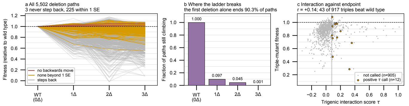
Figure 5: All 5,502 measured deletion paths through the pcl6Δ pcl7Δ screen, the step at which each route stops climbing, and trigenic interaction against endpoint fitness. Generated by experiments/010-kuzmin-tmi/scripts/pcl6_deletion_paths.py .
