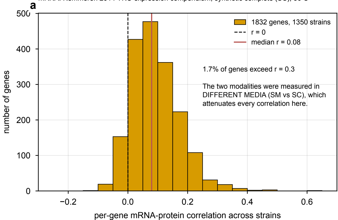
Figure 13: Per-gene correlation across strains between the Messner 2023 knockout proteome and the Kemmeren 2014 knockout expression compendium, over the 1,832 genes and 1,350 deletion strains they share. A narrow lump barely off zero: mRNA and protein levels for the same gene move largely independently across this panel. The few high- r genes are dominated by the strain in which that gene is itself deleted, which drives both its transcript and its protein toward zero and manufactures a correlation from one point.
