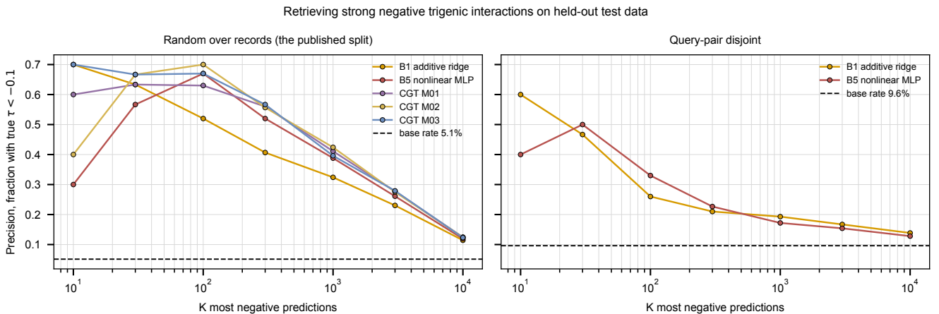
Figure 3: Precision at K for retrieving records with true \tau < -0.10 , on both splits, with the base rate marked.
