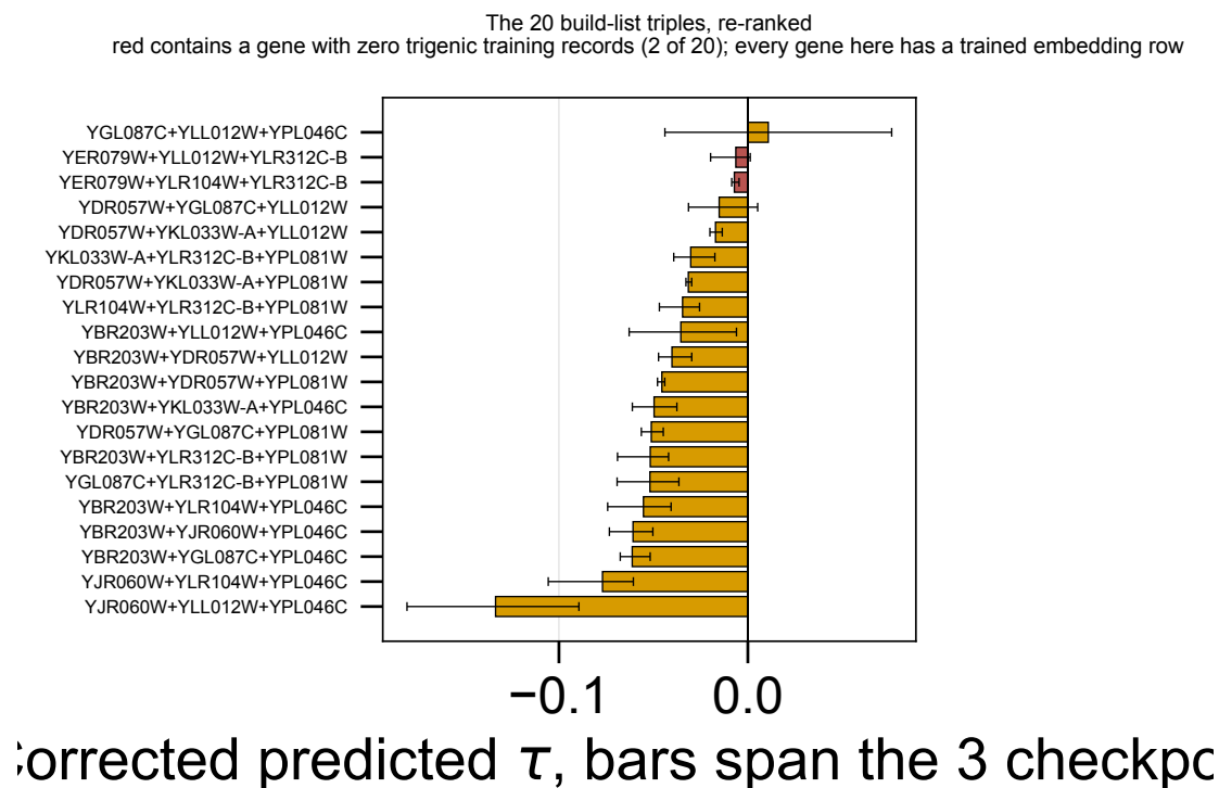
Figure 2: The 20 build-list triples re-ranked, bars spanning the three checkpoints. Red marks a triple containing a gene with zero trigenic training records, which on this list is YER079W alone.
