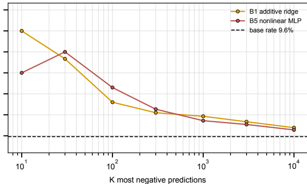
Query-pair disjoint
