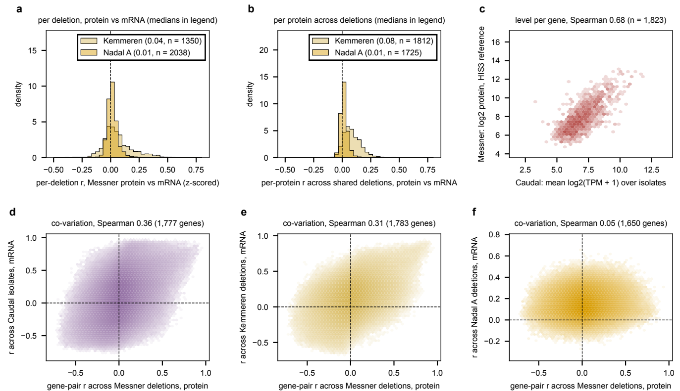
Figure 14: The Messner 2023 knockout proteome against three expression panels. a , per shared deletion, the Pearson between its protein and mRNA \log_2 ratios (z-scored per gene across strains) for Kemmeren and for Nadal-Ribelles A. b , per protein, the Pearson across shared deletions. c , abundance level per gene, protein in the HIS3 reference against mean expression over the Caudal isolates. d-f , gene-pair co-variation: the correlation of two genes across Messner's deletions (protein) against the same pair across Caudal's isolates, Kemmeren's deletions and Nadal-Ribelles A's deletions (mRNA), log-count density. Generated by proteome_expression_covariation.py.
