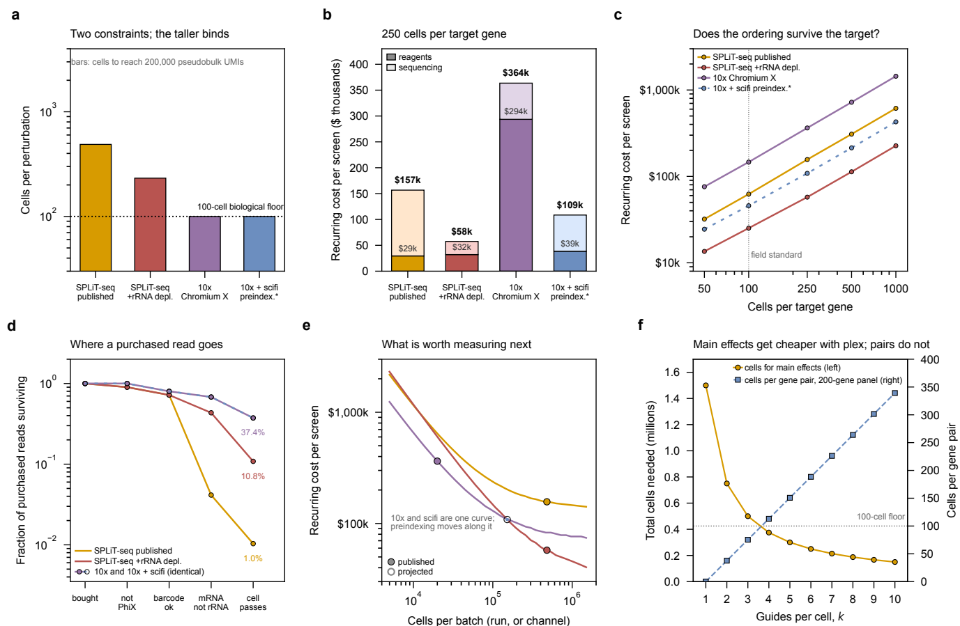
Figure 10: Six views of one decision: which platform to run. Color is the platform in every panel and only ever the platform, so the key is learned once; where a panel needs a second dimension it uses lightness within the platform's own color, or hatching against white. The asterisk marks the projected row, drawn inside the panels because a screenshot loses a caption. All four columns are 6,000 target genes in one environment at UIUC rates; panels (a), (b), (d) and (e) are priced at 250 cells per target gene. (a) Cells per perturbation, under two independent constraints (section 4.3): the depth requirement, i.e. how many cells it takes to accumulate 200,000 pseudobulk UMIs at each platform's per-cell yield, against the 100-cell biological floor below which cell-cycle and metabolic state are not averaged out. The taller bar binds, and the floor binds for every deeper platform, so past a few hundred UMIs per cell the design is limited by how many cells must be observed rather than by how deeply each is read. The preindexed column is identical to the 10x column here, which is the point of showing it: preindexing buys cells per dollar, not UMIs per cell, and is invisible to every statistical panel in this document (fig. 8d). (b) Where the recurring money goes , split into the two terms that carry the message: the platform's own color for reagents – barcoding, library preparation and, for the split-pool columns, sublibrary preparation – and its pale companion for sequencing. Sublibrary prep sits inside the reagent term rather than being drawn separately, which is how table 16 groups the same money and is also the only legible choice: at $2,970 of a $156,670 screen it is under 2% of a bar, and a band four points tall cannot carry a pattern. The dominant term moves : sequencing is 81% of split-pool spend, while for 10x it is 19% and library preparation 81%, because a genome-scale screen consumes 137 channels at $2,143 each. These are different cost structures, and an optimization that helps one (rRNA depletion, worth ~$99,000 here) does nothing for the other. Preindexing takes the 137 channels to 18 and the column to $109k, and in doing so moves that platform's dominant term onto sequencing as well – reagents 36%, sequencing 64% – but with no rRNA left to deplete. (c) Whether the ordering survives a change of target. Panel (b) prices one design; this sweeps 50 to 1,000 cells per target gene. The ordering is stable across the whole range, so the platform choice is not an artifact of the 250-cell point, and the vertical rule marks the 100-cell field standard the recommendation is actually made at. (d) What happens to a purchased read , stage by stage, and this is where the reagent comparison and the cost comparison part company. Split-pool reagents are ~22× cheaper per cell than droplet and it still loses end to end; the reversal is entirely here. Of 100 reads bought for a split-pool run, 10 are PhiX spike or unresolvable barcode, 94 of the remainder are ribosomal, and three quarters of the cells they came from are then discarded – 1.0 read in 100 survives all four tolls. Depletion takes that to 10.8, and both droplet columns reach 37.4. The two droplet lines coincide exactly at every stage , which is worth seeing: preindexing touches no term in this panel. (e) What is worth measuring next. Every platform here has exactly one number that is both uncertain and load-bearing, and for all of them it is the same field – cells barcoded per protocol run, or cells recovered per channel – so they share an axis. The two are not equally worth measuring. Droplet cost is reagents and reagents are per batch, so its curve falls steeply and keeps falling; split-pool cost is sequencing, which does not depend on this number at all, so its curve flattens almost at once and learning that yeast tolerates a denser RT well buys little past a few hundred thousand cells per run. 10x and scifi are one curve, and preindexing is a move along it rather than a move to a different one. (f) What multiplexing buys as guides per cell k rises. Left axis: total cells needed to hold main-effect precision across 6,000 genes falls as 1/k , from 1.5 M cells at k = 1 to 0.15 M at k = 10 , because every cell reports on k genes at once. Right axis: what that same cell budget delivers for one named gene pair if the library is restricted to a 200-gene panel, which grows roughly linearly in k and crosses the 100-cell floor near k = 4 . Multiplexing alone does not open up epistasis – run the same calculation over all 6,000 genes and coverage per pair falls by (200/6000)^2 \approx 1/900 , to well under one cell per pair at any k , because the pairs to be covered grow quadratically while the pairs a cell reports grow only as k^2 . Restricting the panel is what makes pairs measurable and 25 multiplexing is what then makes it affordable; neither substitutes for the other. The scifi column is a projection throughout. It changes exactly one parameter of the 10x column – cells recovered per channel becomes Datlinger et al.'s measured 151,788 rather than the UIUC baseline of 20,000 – and per-cell depth
