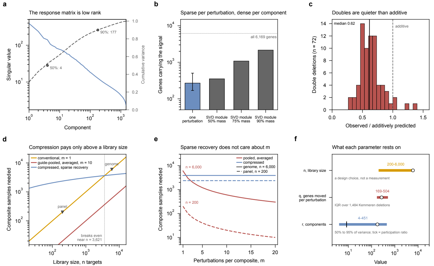
Figure 7: The yeast response matrix is compressible, and compression is still the wrong tool for a focused screen. All panels are Kemmeren et al.’s 1,484 single deletions [22] and Sameith et al.’s doubles [23], the same compendia as fig. 6. Color is the design throughout: amber conventional, red pooled-and-averaged, blue compressed. (a) Singular spectrum of the effect matrix (left axis) and cumulative variance (right). Four components carry half the variance and 177 carry 90%; the participation ratio, a cut-off-free reading of the same spectrum, is 8.4. (b) Two sparsities, and only the first is the one the bound uses. One perturbation moves 269 genes of 6,169 (bar, with interquartile range); a singular component needs 2,155 to carry 90% of its mass, because an SVD component is dense by construction. The grey bars are an upper bound on what a sparse factorization would need, not a measurement of it. (c) The additivity assumption, tested. For each double deletion whose two singles were profiled by the same lab, the slope of observed response on additively predicted response, over genes either vector moves. Additive is 1; the median is 0.62. Restricting to moved genes matters – a correlation over all 6,000 would be dominated by the \sim 5,700 sitting at zero in both vectors and would report near-perfect additivity for any pair of sparse vectors. (d) Composite samples needed against library size, at the measured q and r . Every constant here is 1: Yao et al. state an order, and a compressed-sensing constant depends on the measurement ensemble and the recovery guarantee wanted, so the panel compares shapes – flat in n against linear in n – and the crossing, whose location moves with the constant but whose existence does not. (e) The same quantity against perturbations per composite. The compressed curves are horizontal because sparse recovery’s requirement does not depend on m at all, only on what is being recovered; that is the whole difference between the two decodings. (f) What each parameter rests on. n is a design choice; q is an interquartile range over 1,484 measured deletions; r has no single value because the spectrum has no knee, so the bar spans the 50% and 95% variance cuts and the tick marks the participation ratio. Generated by experiments/019-perturb-seq-costing/scripts/plot_compression.py , from compression_analysis.py .
