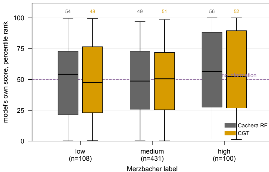
Fig 4 – score by class, as percentile rank
