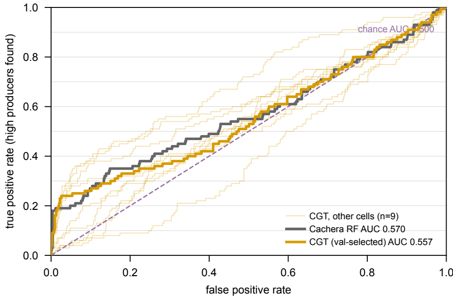
Fig 5. Threshold-free, and it goes marginally to their RF: AUC 0.570 vs CGT's 0.557. Both near the 0.500 chance line, because AUC integrates over the whole ranking where neither model has much. The honest summary is metric-dependent: CGT wins global Spearman, RF wins AUC, precision@k is a wash, and no gap is large.
