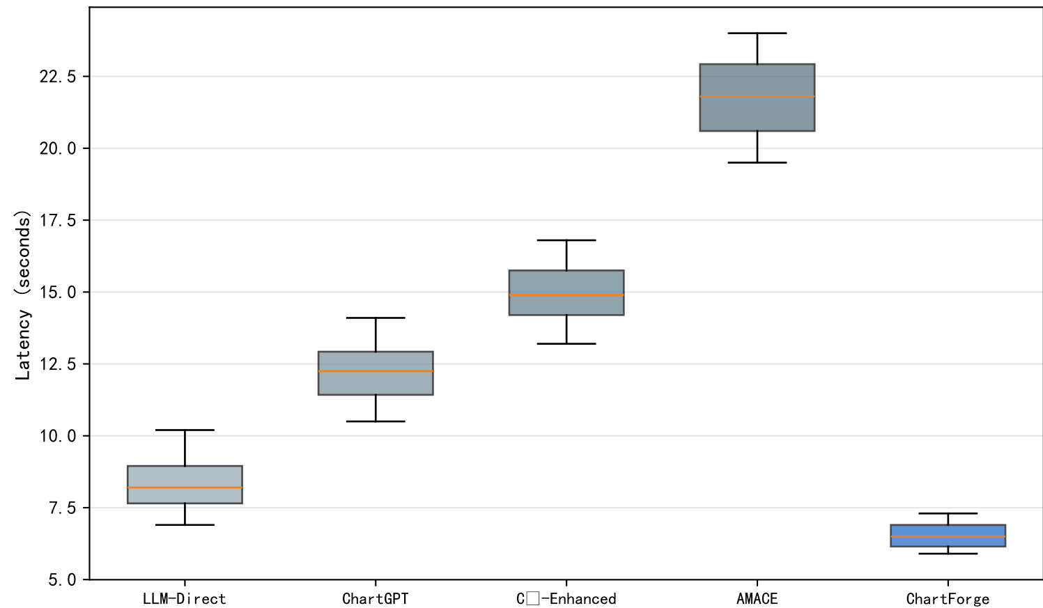
Generation Latency Distribution by Method
