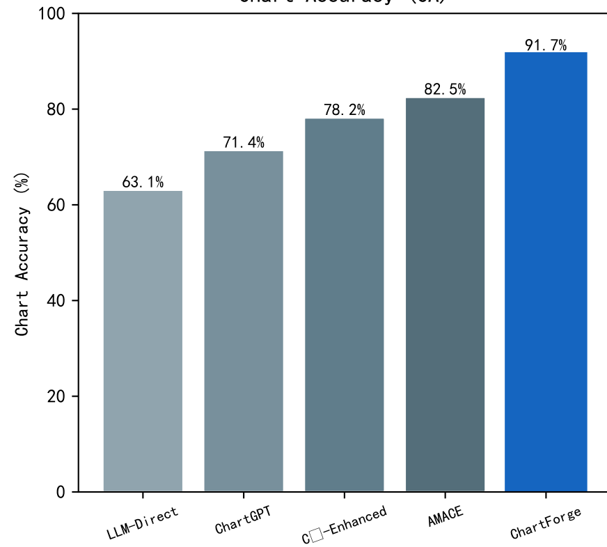
Chart Accuracy (CA)
