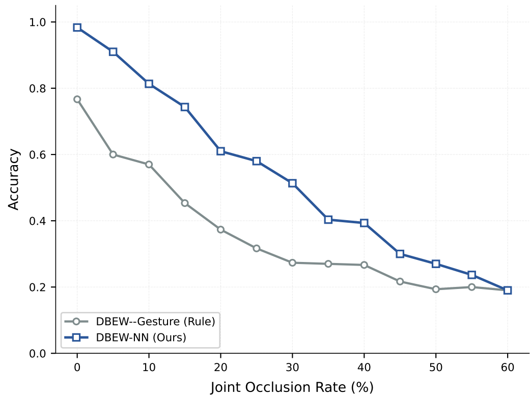
Occlusion Robustness
