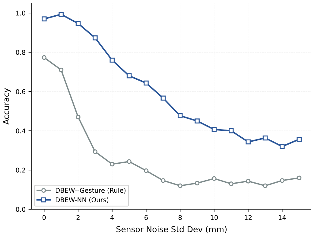
Noise Robustness
