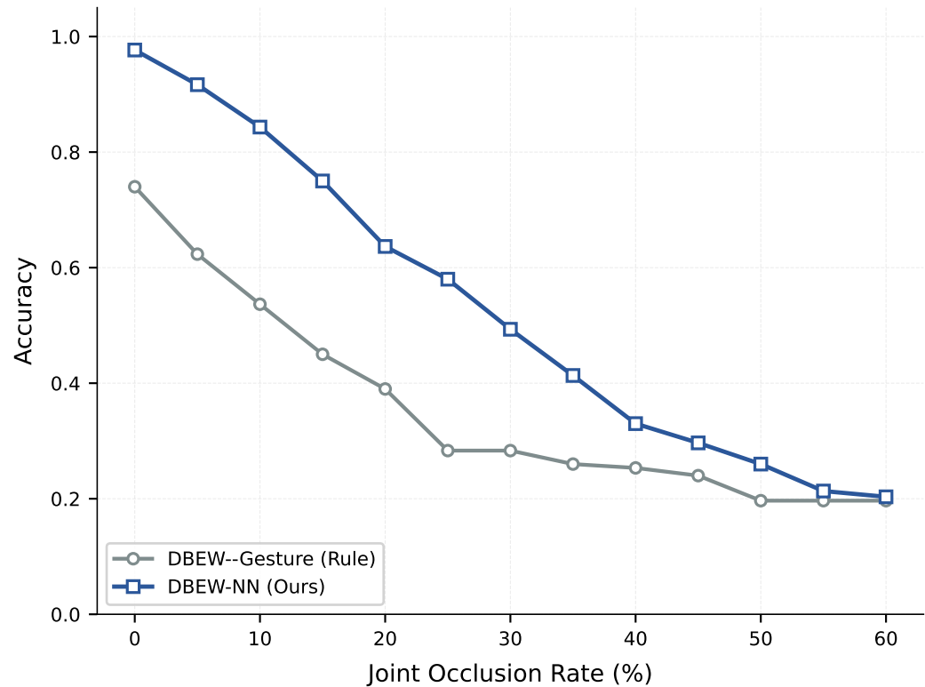
Occlusion Robustness
