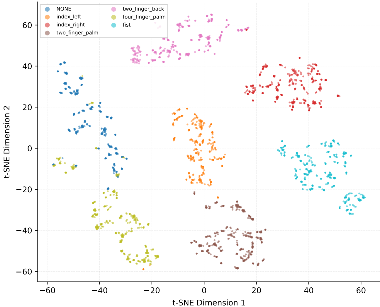
DBEW-NN Feature Space (t-SNE Projection)
