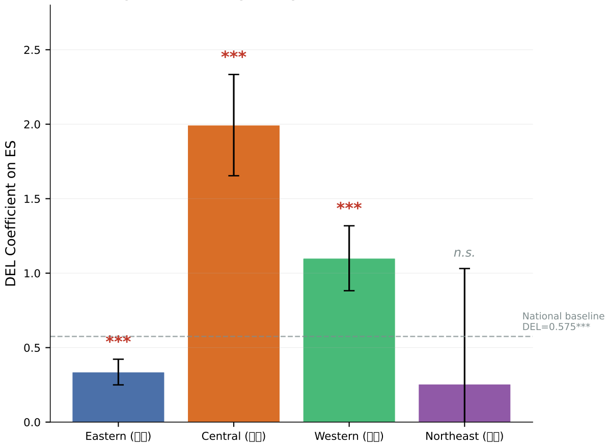
Regional Heterogeneity: DEL→ES Coefficients
