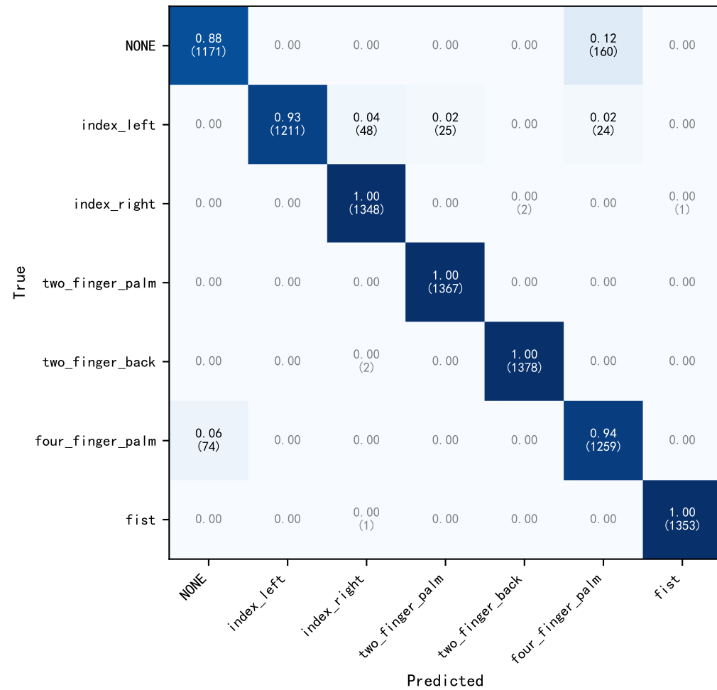
DBEW-NN (CNN+Attention)
