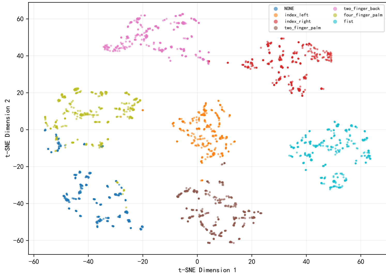
DBEW-NN Feature Space (t-SNE)
