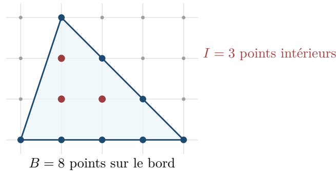
Figure D.8: Pour ce triangle, I = 3 , B = 8 et \mathcal{A} = 3 + 8/2 - 1 = 6 .
