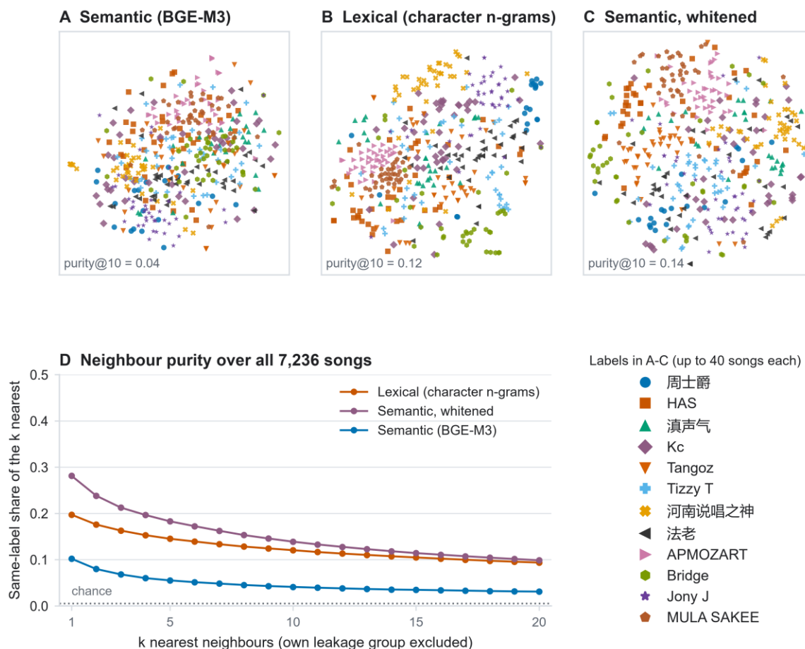
Fig. 5 The same songs in three representation spaces, and how often a song's nearest neighbours share its source-credit label. Panels A–C are t-SNE layouts of one fixed set of 442 songs from the twelve labels with the most songs, at most one song per leakage group, in the BGE-M3 space (A), the character 2–5-gram TF–IDF space (B), and the BGE-M3 space after within-author whitening fitted on songs by every other label (C). One seed and one perplexity are used throughout; cluster sizes and the distances between clusters carry no meaning (van der Maaten and Hinton 2008). Panel D is the measurement the layouts gesture at, over all 7,236 songs and without any projection: for k from 1 to 20, the share of a song's k nearest cosine neighbours, excluding its own leakage group, that carry its label. The whitened curve is fold-wise, so no song is scored in a space fitted on itself. The dotted line is the chance level implied by label sizes.
