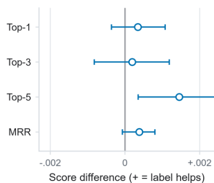
Fig. 4 Prediction of the next dictionary-estimated written line-ending family on the strict terminal-Han population of corpus v2. Panel A compares global frequency, first-order Markov, flat context, and hierarchical context with and without the source-credit label across 51,516 leakage-safe events in 1,064 held-out songs; whiskers are 95% song-cluster bootstrap intervals from 2,000 replicates. Panel B separates continuation from family-switch events. Panel C plots four paired score differences for the model with versus without the label; three intervals cross zero and the largest difference, Top-5, is +0.0015.
