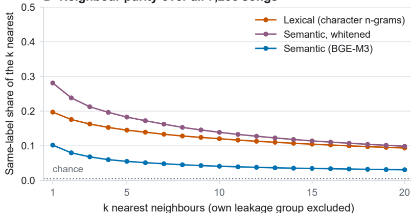
D Neighbour purity over all 7,236 songs
