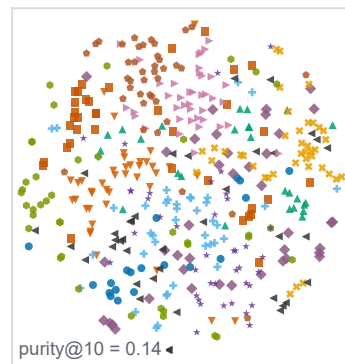
C Semantic, whitened
