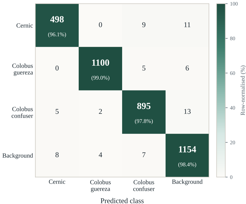
V12 validation confusion matrix (n = 3 717, accuracy = 98.12%)
