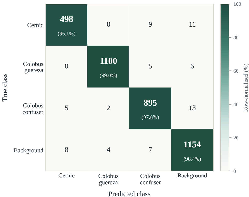
V12 validation confusion matrix (n = 3 717, accuracy = 98.12%)
