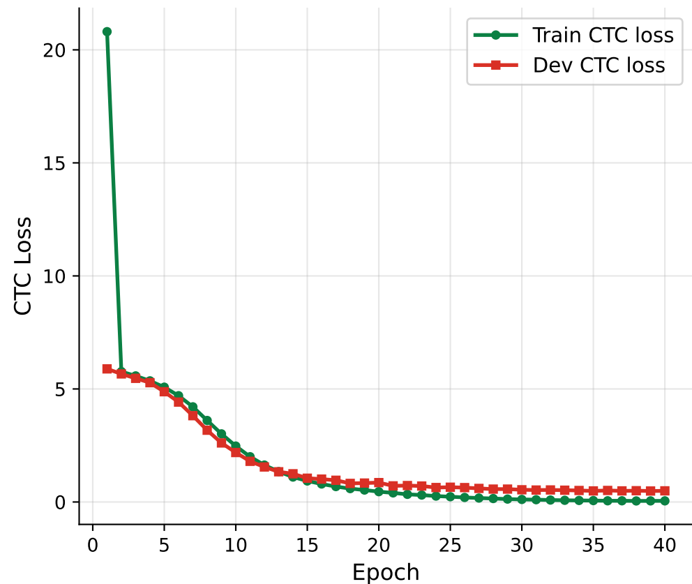
Conformer + CTC — Loss Curves
