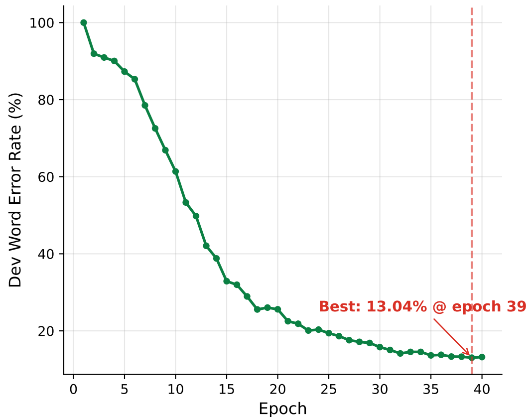
Conformer + CTC — Dev WER
