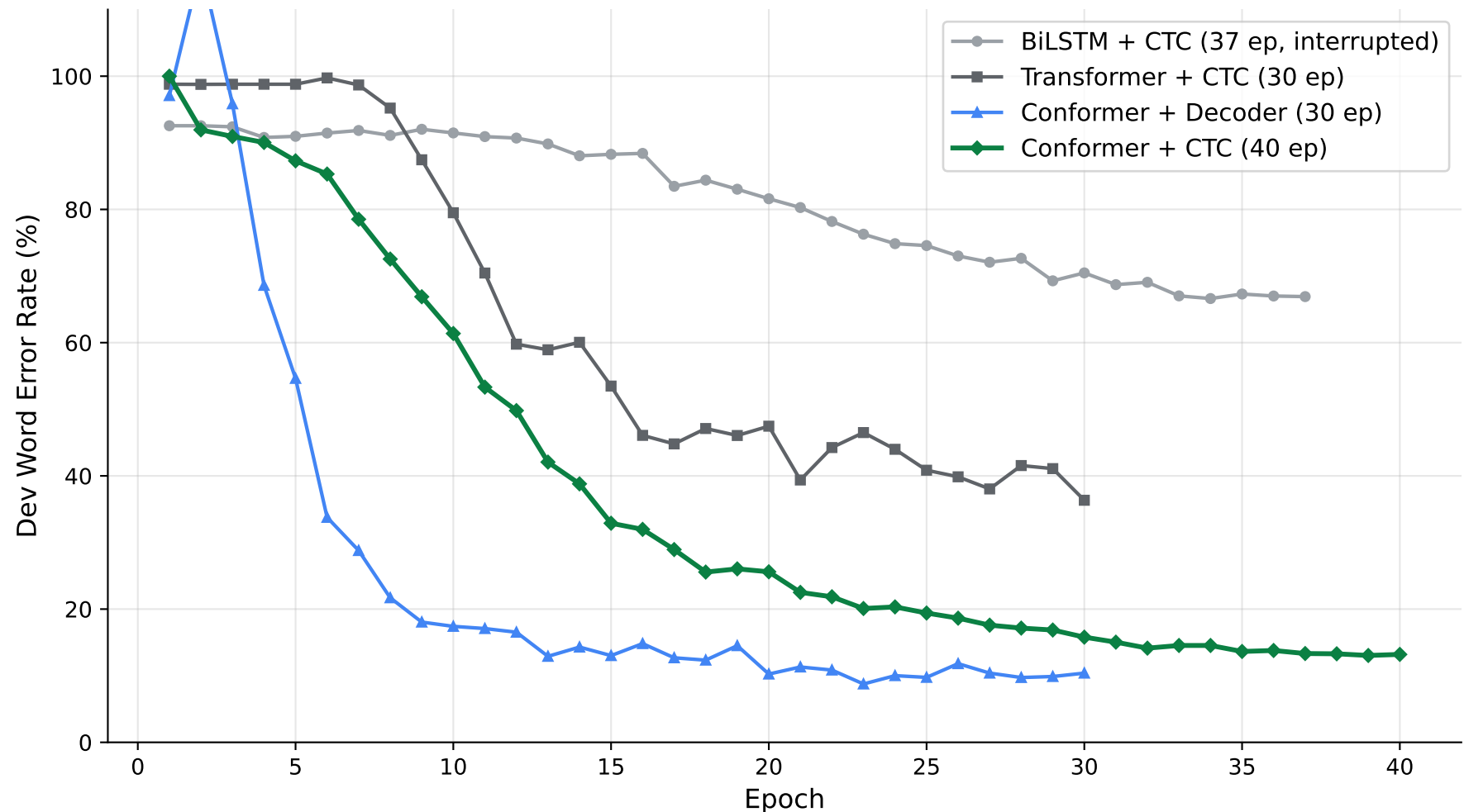
Dev WER Convergence Across All Four Architectures
