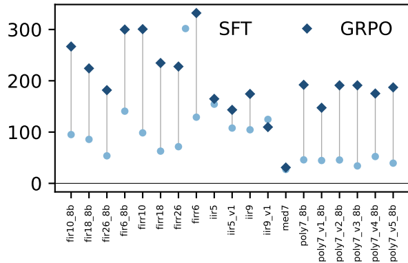
Penalized equal-sample F_{max} (MHz)
