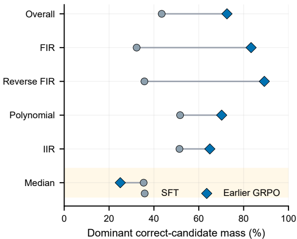
(a) Probability concentration
