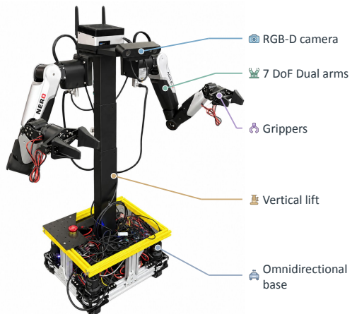
Fig. 3. YOR robot platform used in our experiments, equipped with an RGB-D camera, dual arms with grippers, a vertical lift, and an omnidirectional base.
