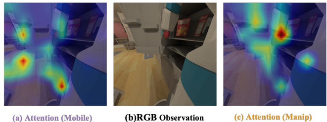
Fig. 4. Query attention visualization. (a) Mobile Query attention, (b) the RGB observation, and (c) Manip Query attention.
