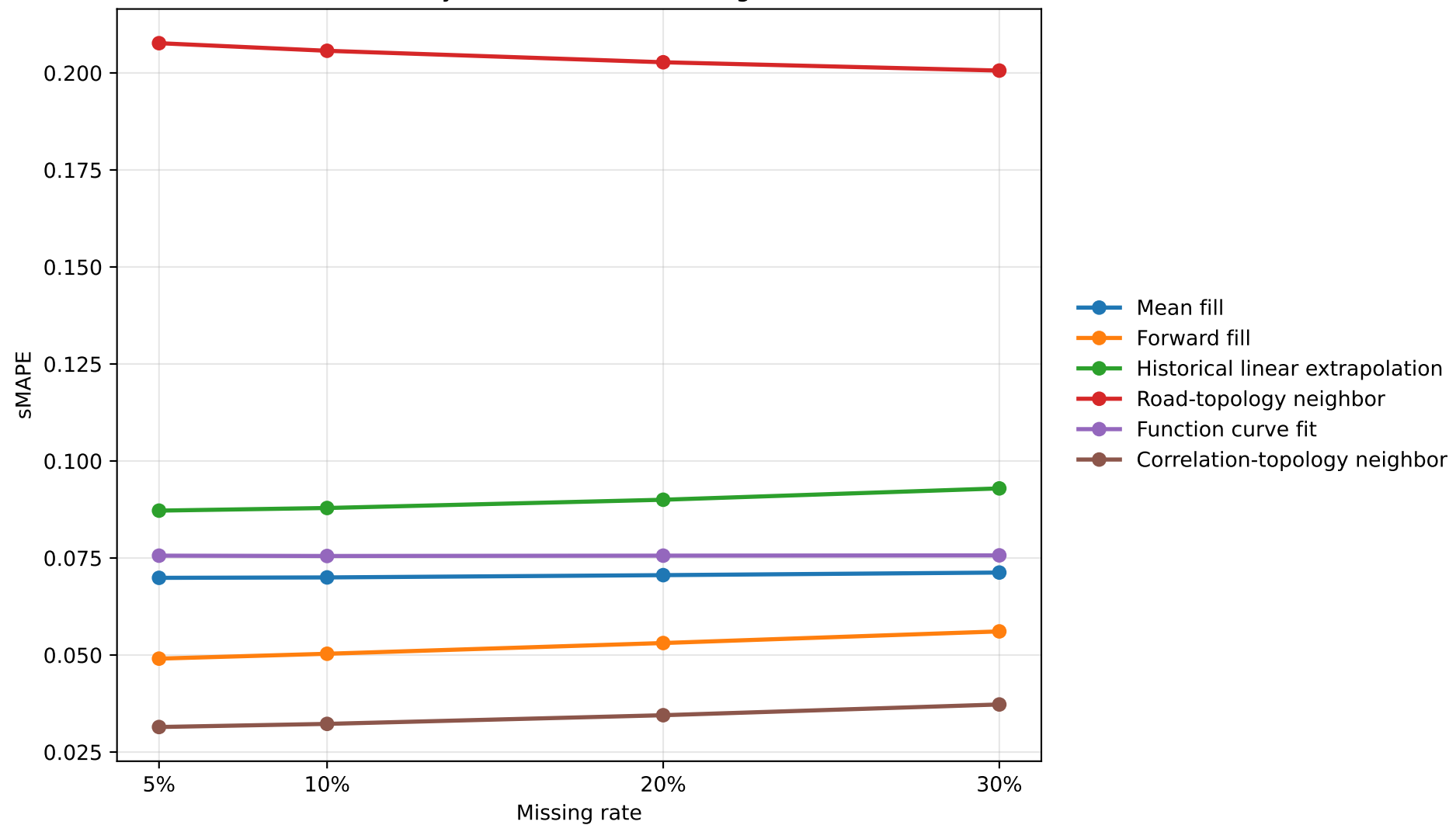
sMAPE by method across missing rates
