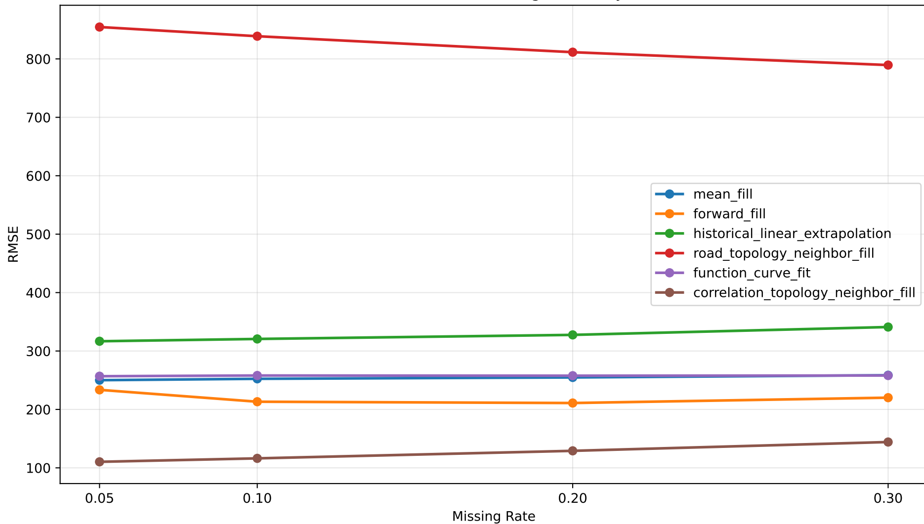
Structured Node Subset Outage RMSE by Method
