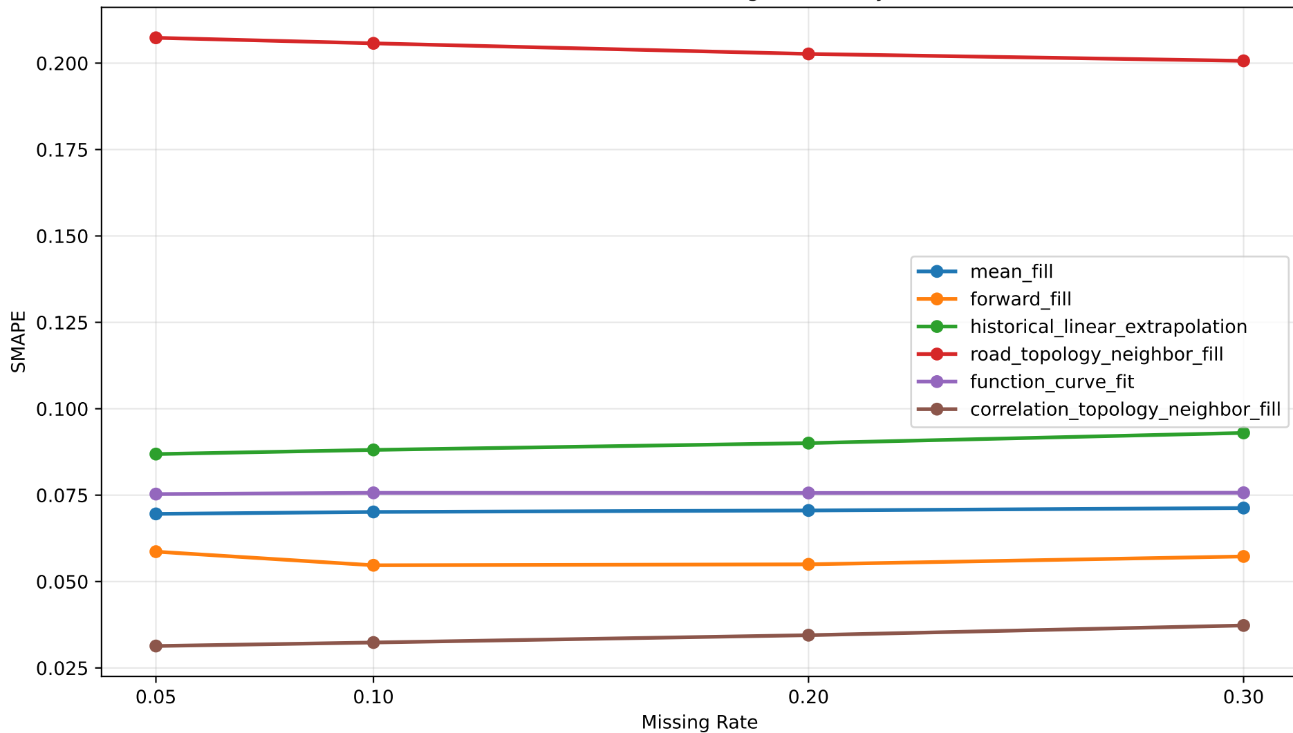
Structured Node Subset Outage sMAPE by Method
