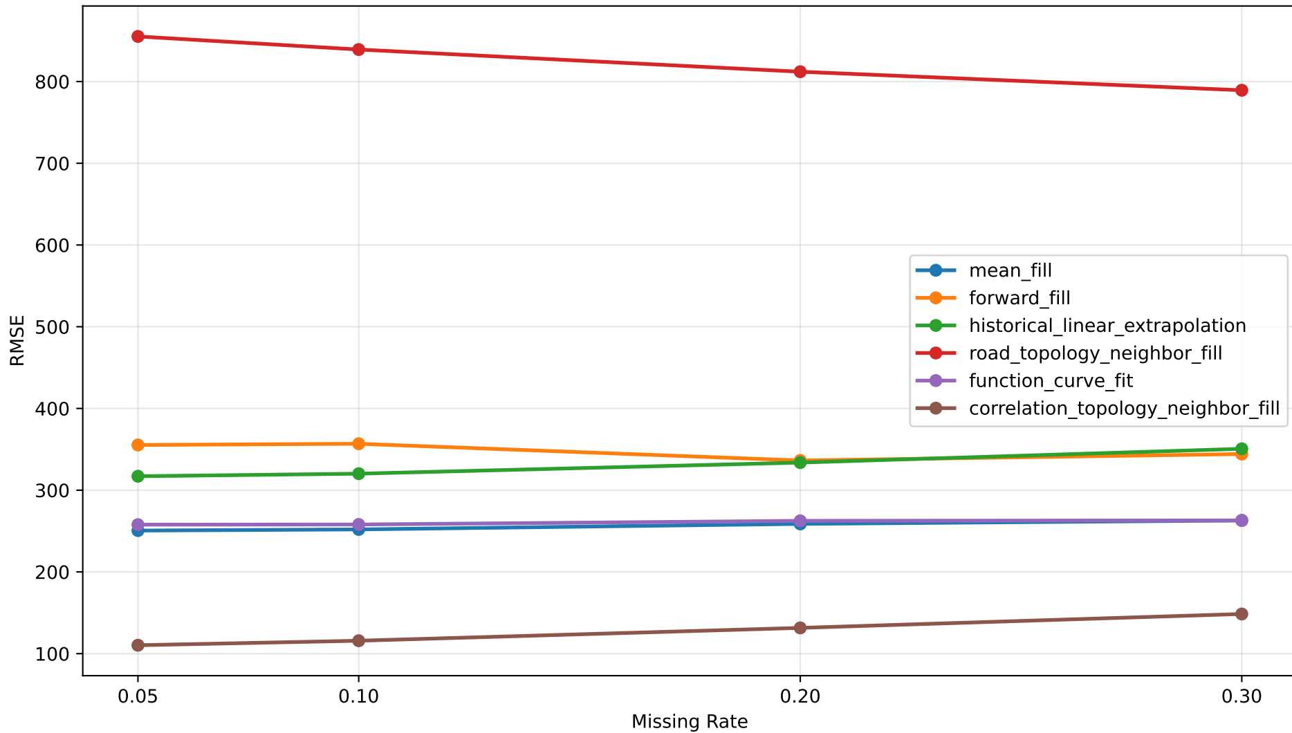
Structured Temporal Block RMSE by Method
