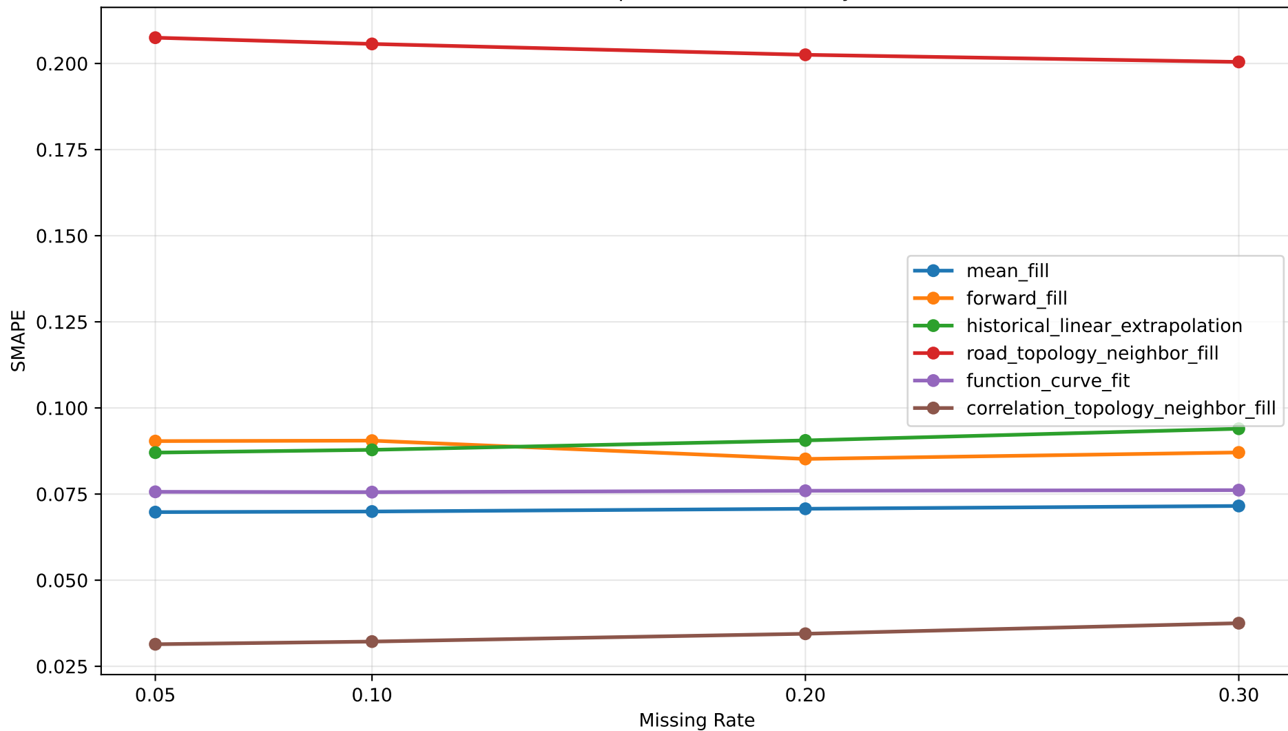
Structured Temporal Block sMAPE by Method
