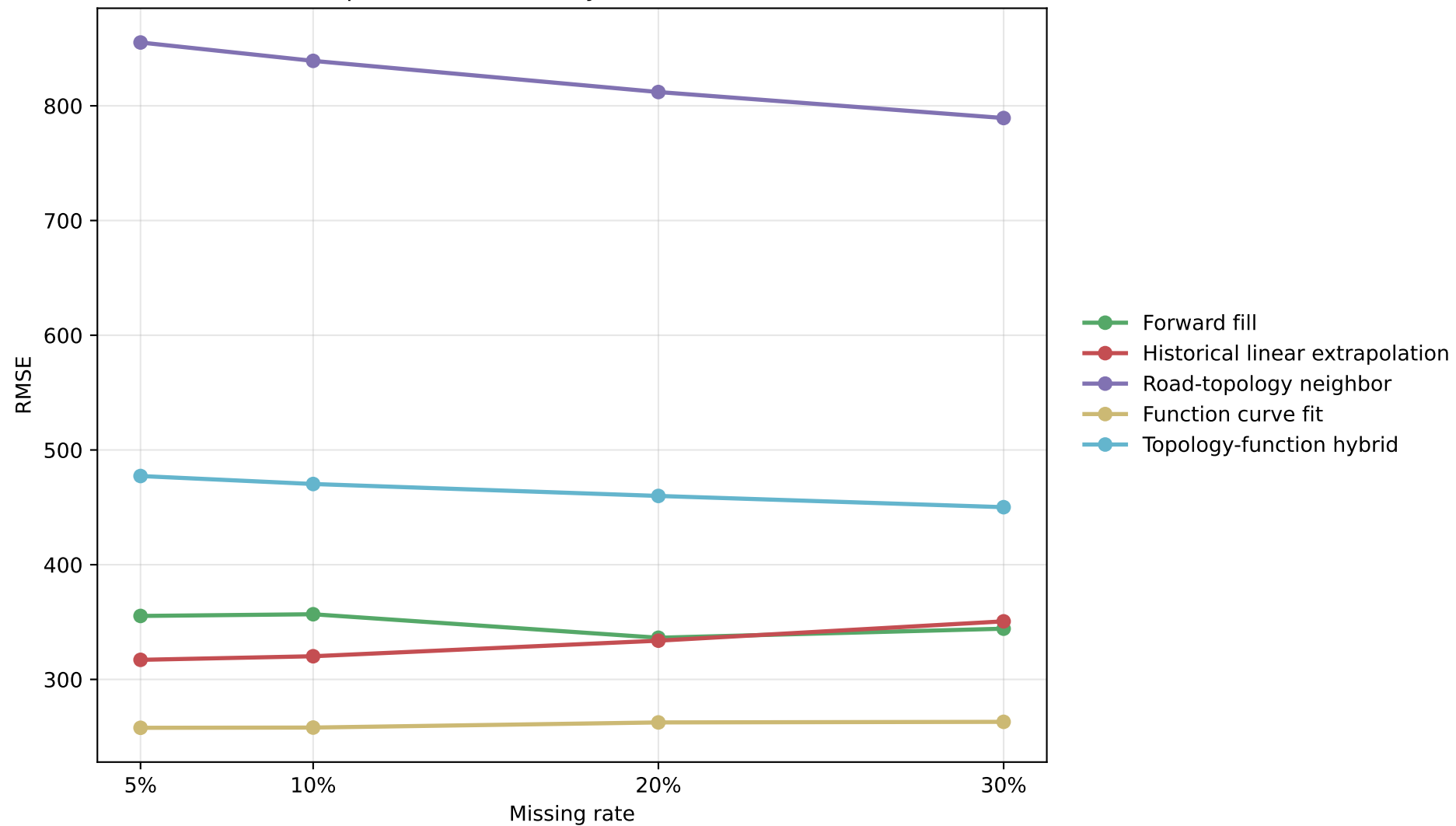
Node temporal block RMSE by Method (Non-zero Zoom)
