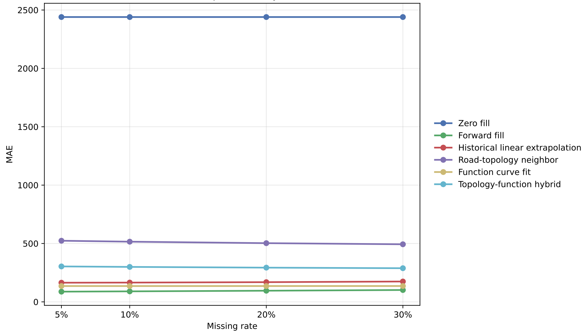
Global MCAR point MAE by Method
