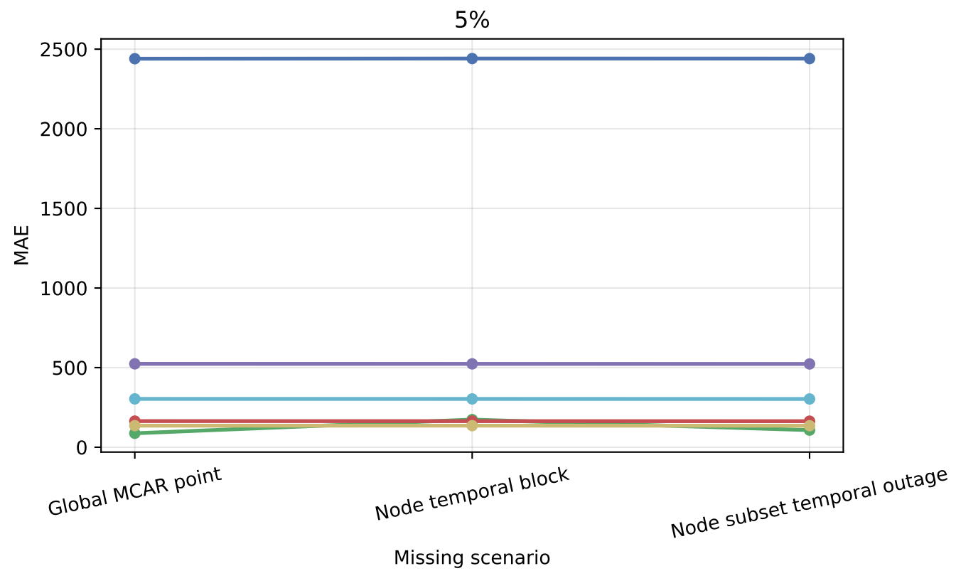
Scenario Comparison MAE by Method
