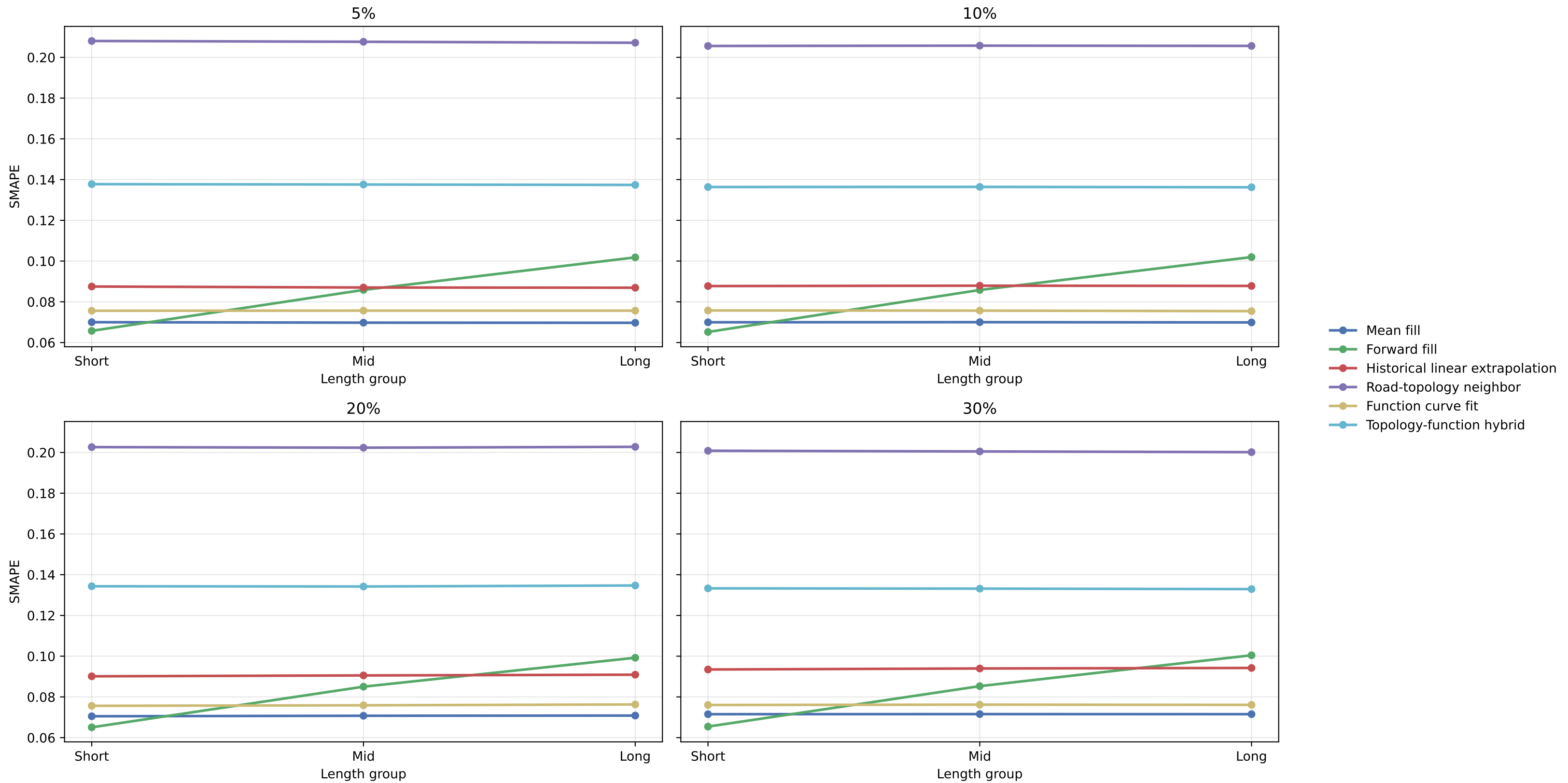
Node temporal block SMAPE by Length Group
